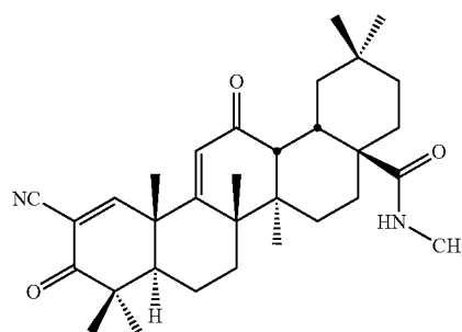
CDDO-MA (TP-224)
