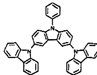
Comparative Compound 3
