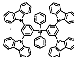
Comparative Compound 9
