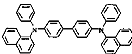
Compound B
