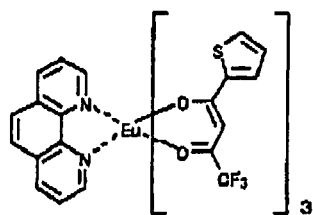
Light-Emitting Material I
