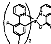
Light-Emitting Material D (466 nm)
