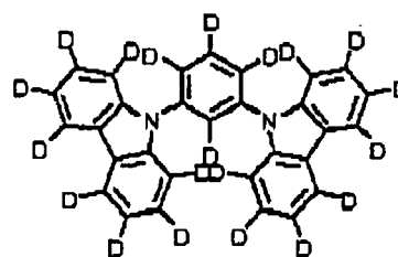
Exemplified Compound (4-6)
