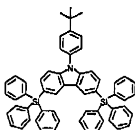
Comparative Compound 7
