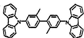
Comparative Compound 4
