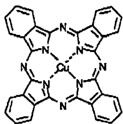
Compound A
