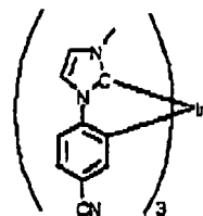
Light-Emitting Material F (458 nm)
