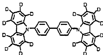
Exemplified Compound (1-3)
