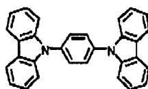
Comparative Compound 5
