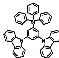
Comparative Compound 6
