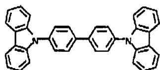
Comparative Compound 1
