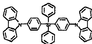
Comparative Compound 8
