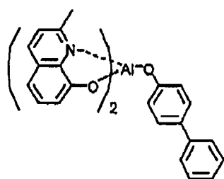
Compound C
