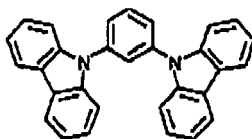
Comparative Compound 2
