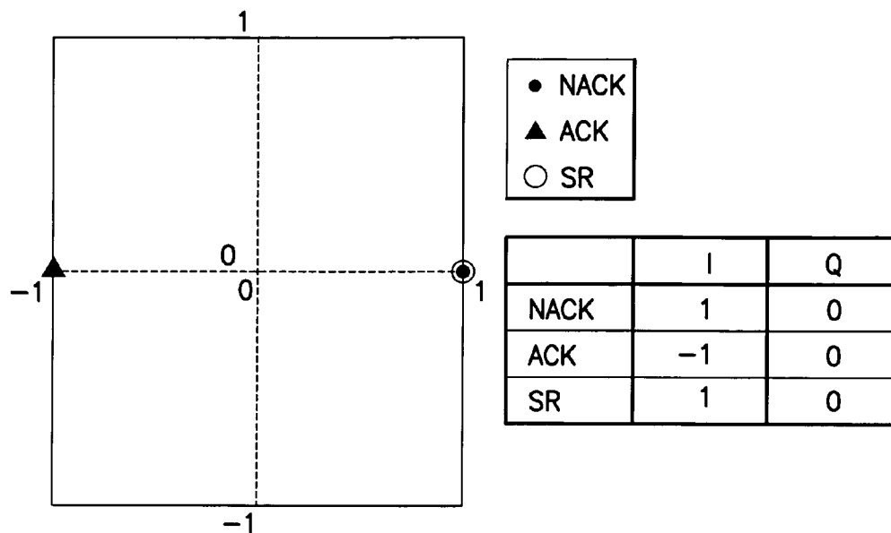
MAPPING OF 1 BIT ACK/NACK CONSTELLATIONS
