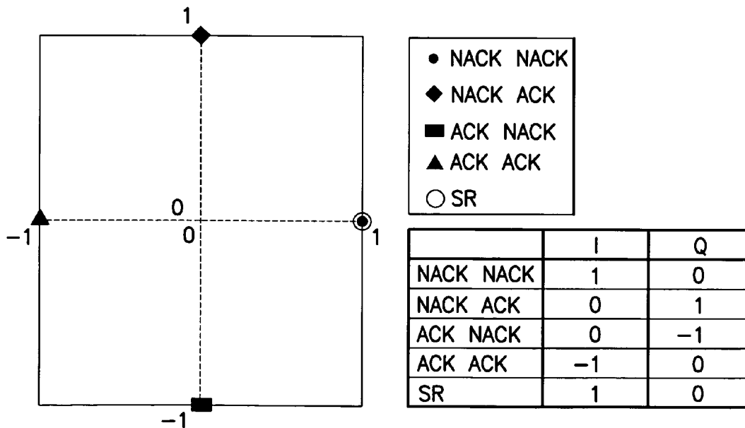
MAPPING OF 2 BITS ACK/NACK CONSTELLATIONS
