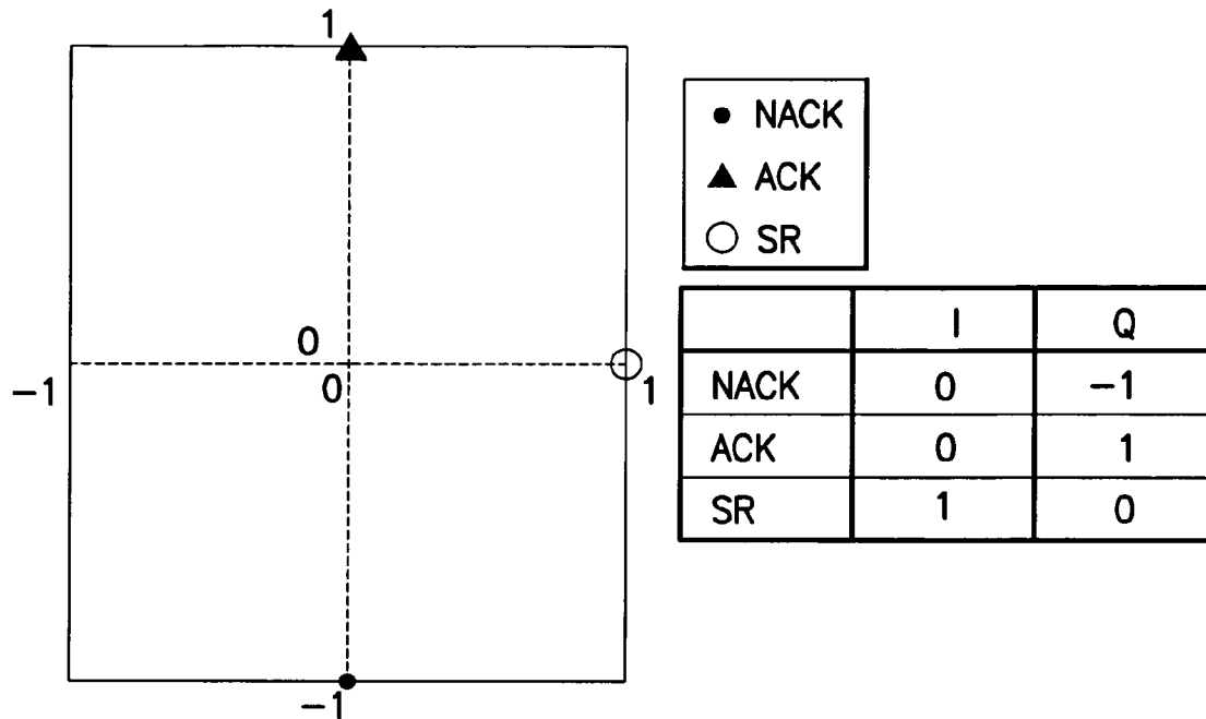
MAPPING OF 1 BIT ACK/NACK CONSTELLATION
