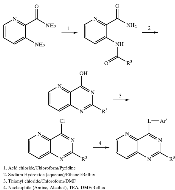
Reaction Scheme 5
