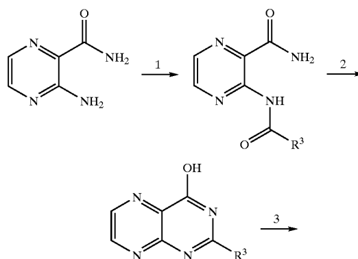
Reaction Scheme 6
