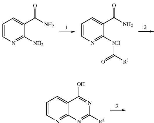
Reaction Scheme 4
