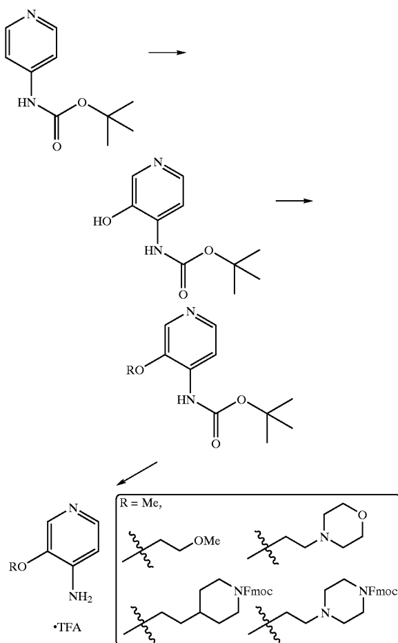
Reaction Scheme 15
