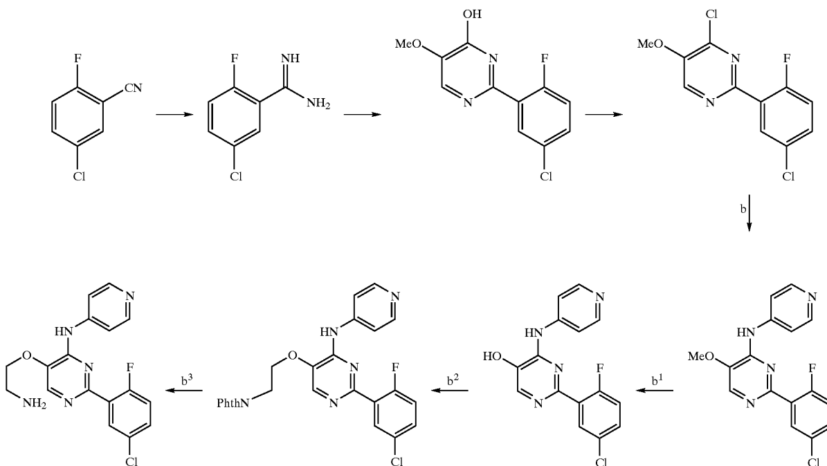
Reaction Scheme 11
