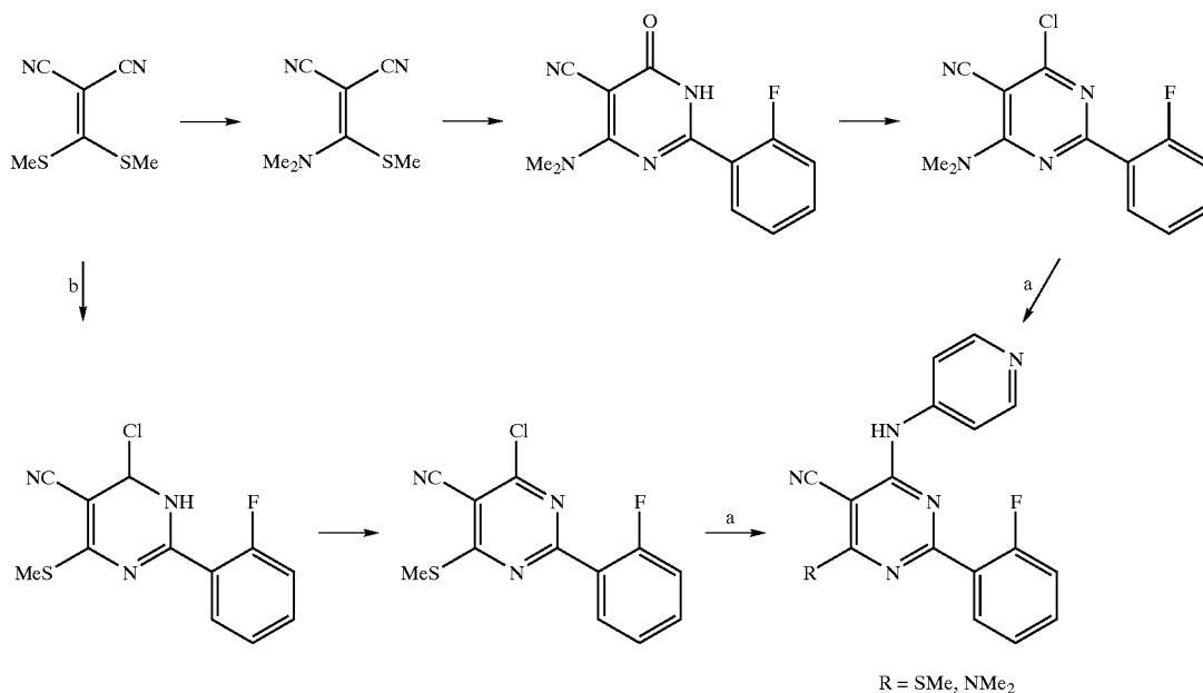
Reaction Scheme 10
