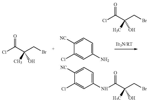
(R)-3-bromo-2-hydroxy-2-methylpropanoic acid R-18
