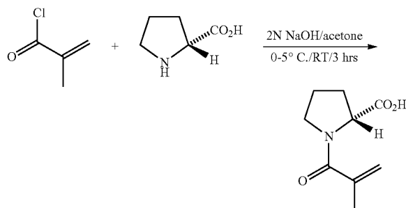
(2R)-1-Methacryloylpyrrolidin-2-carboxylic Acid
