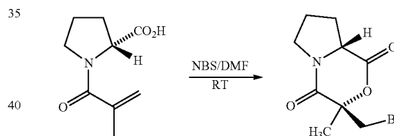
(3R,8aR)-3-Bromomethyl-3-methyl-tetrahydro-pyrrolo[2,1-c][1,4]oxazine-1,4-dione
