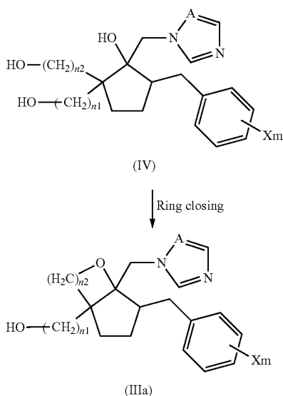
Reaction formula (2)
