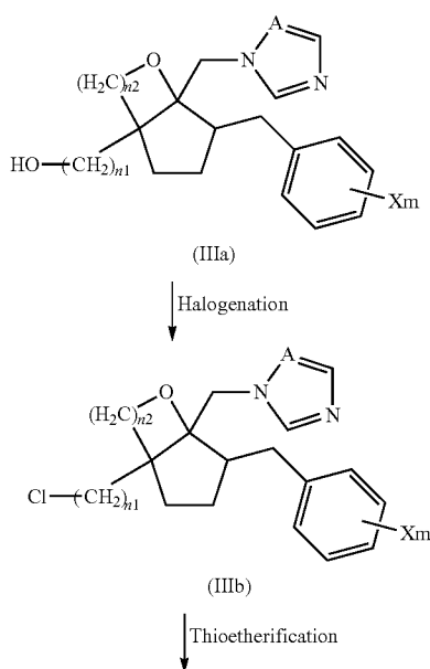
Reaction formula (8)
