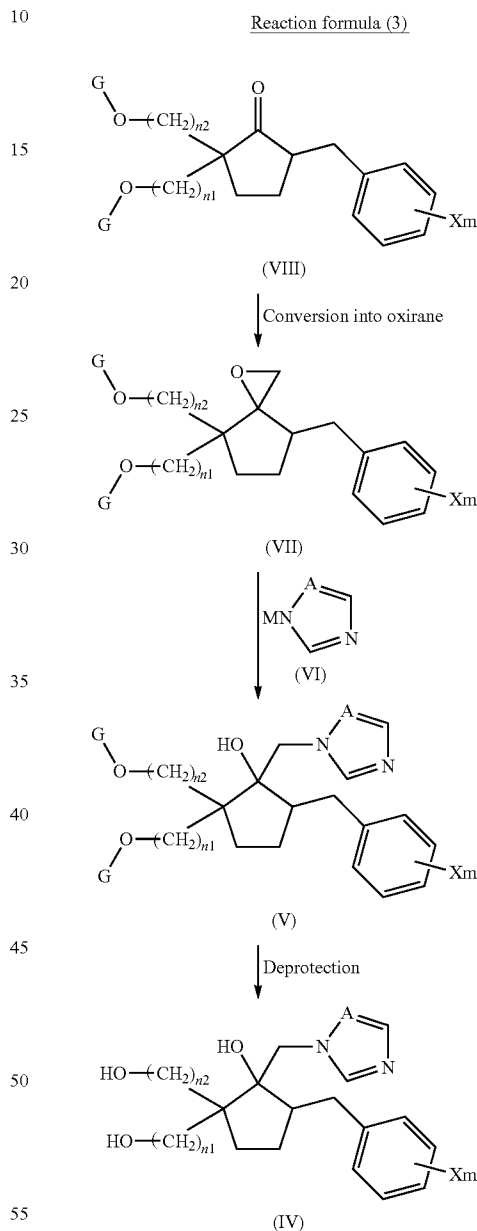
Reaction formula (3)
