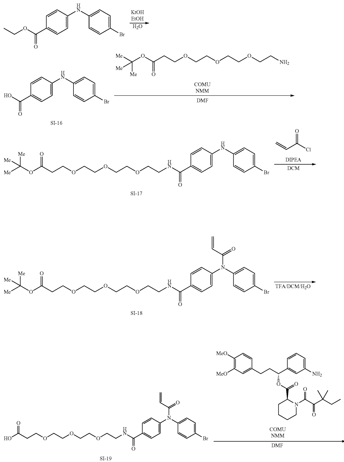
Scheme 6. Synthesis of KB05-SLF
