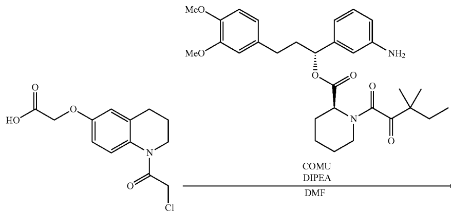
Scheme 4. Synthesis of KB02-PEG0-SLF
