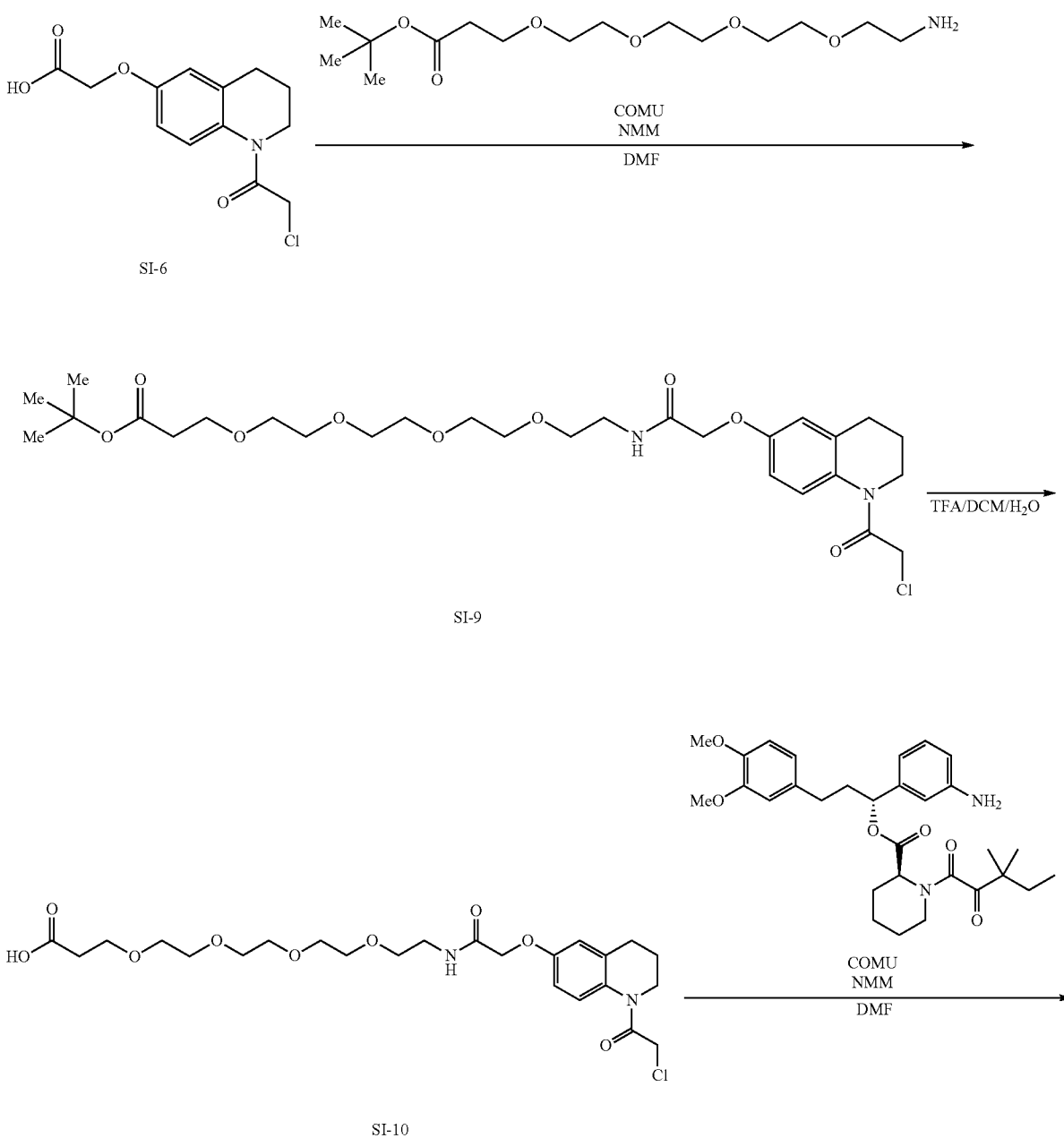
Scheme 3. Synthesis of KB02-PEG4-SLF
