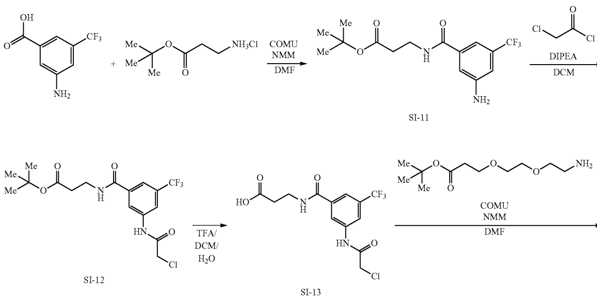
Scheme 5. Synthesis of KB03-SLF
