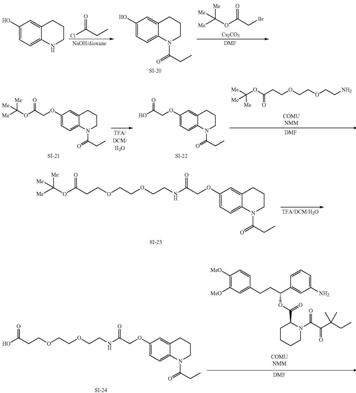
Scheme 7. Synthesis of C-KB02-SLF
