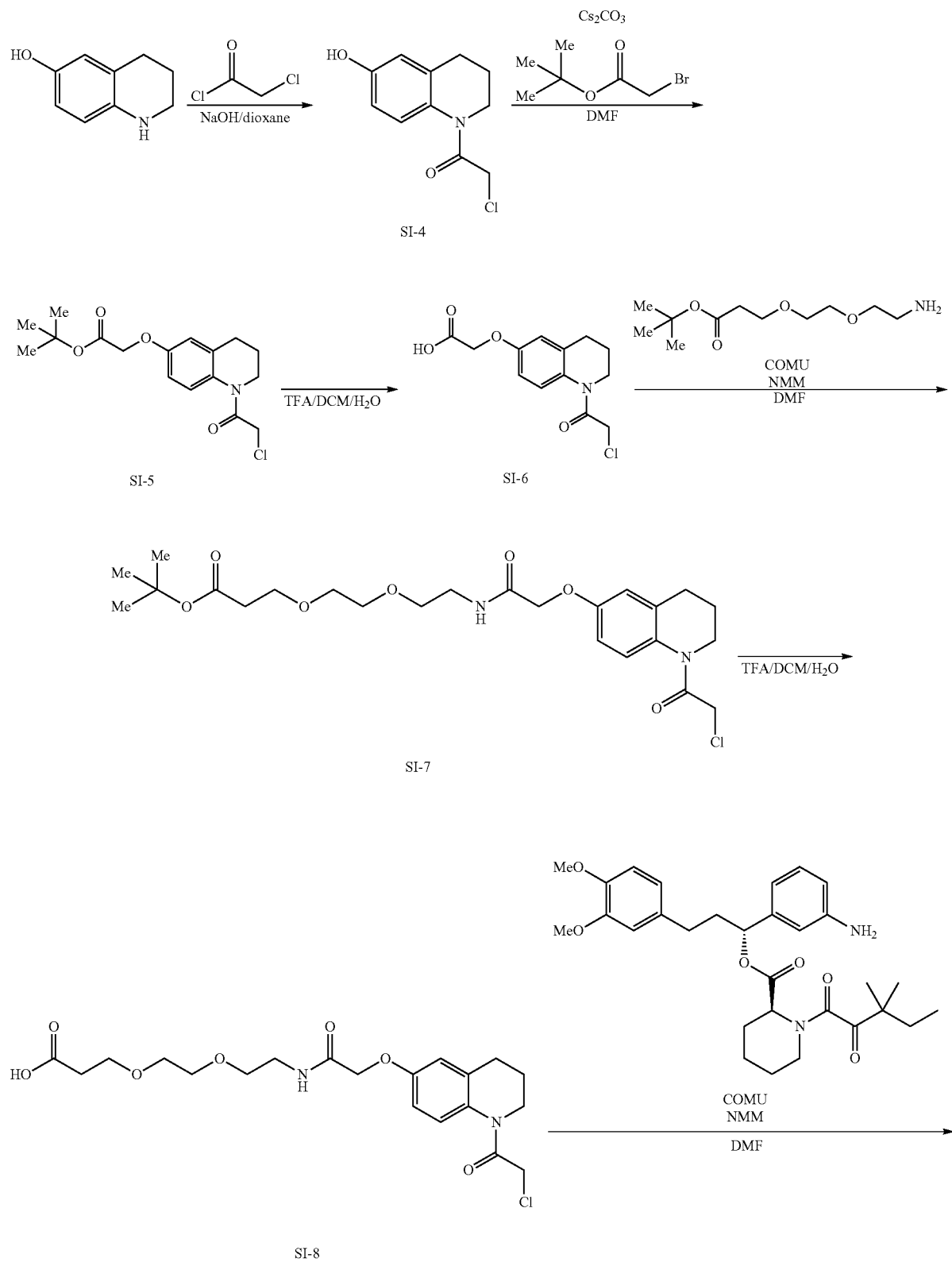
Scheme 2. Synthesis of KB02-SLF
