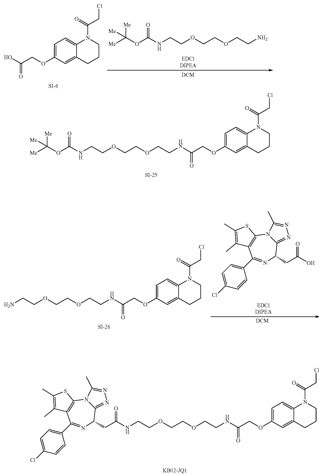
Scheme 8. Synthesis of KB02-JQ1
