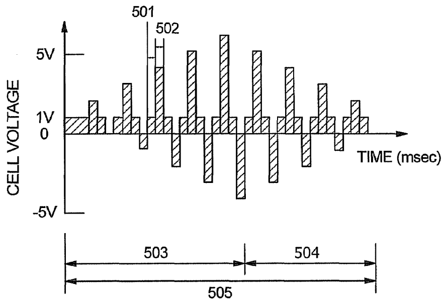
DRIVING WAVEFORM
