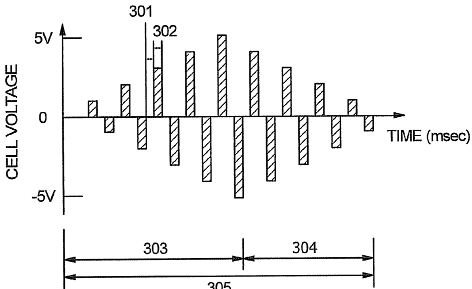
DRIVING WAVEFORM
