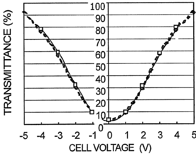
DRIVING RESULT
