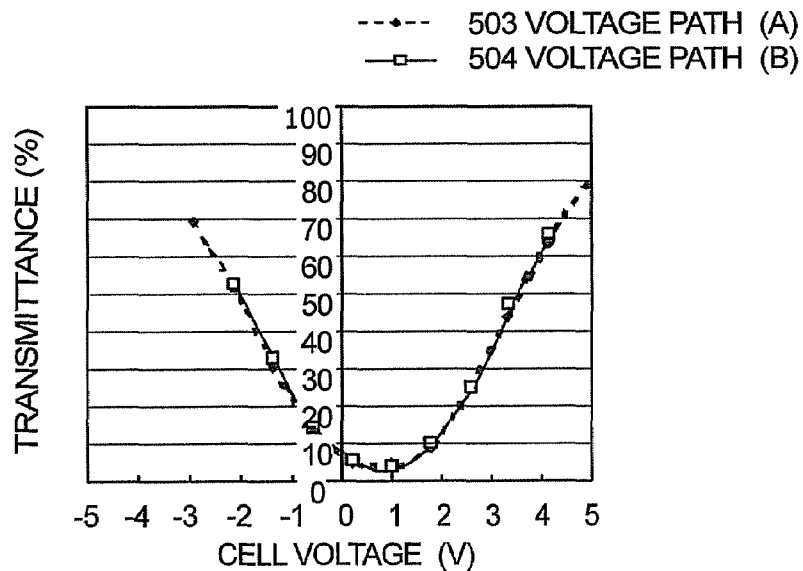
DRIVING RESULT
