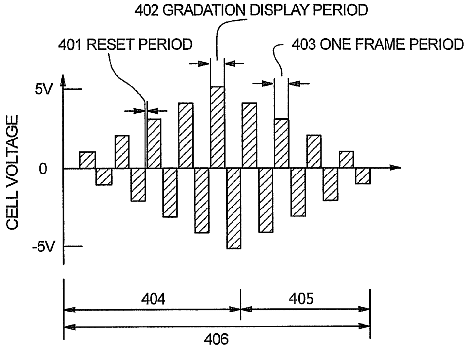
DRIVING WAVEFORM
