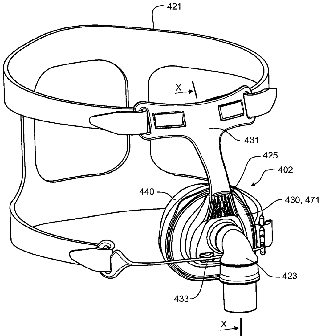
FIGURE 2 (Prior Art)
