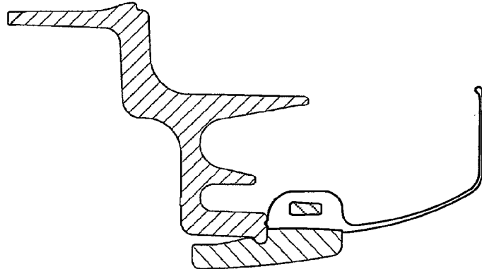
FIGURE 9C (Prior Art)
