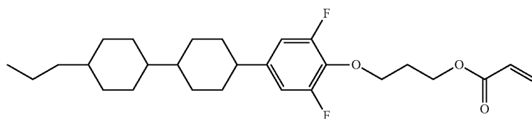
3-(2,6-difluoro-4-(4'-propyl-[1,1'-bi(cyclohexan)]-4-yl)phenoxy)propyl acrylate
