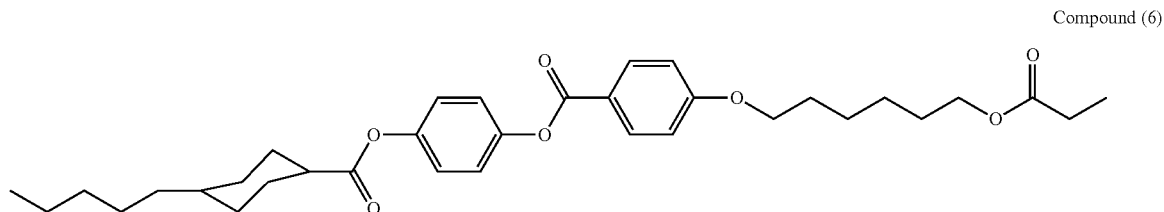
4-((4-pentylcyclohexane-1-carbonyl)oxy)phenyl 4-((6-(acryloyloxy)hexyl)oxy)benzoate
