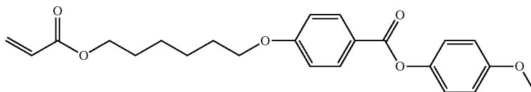
4-methoxyphenyl 4-((6-(acryloyloxy)hexyl)oxy)benzoate
