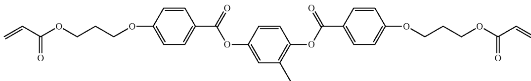
2-methyl-1,4-phenylene bis(4-(3-(acryloyloxy)propoxy)benzoate)
