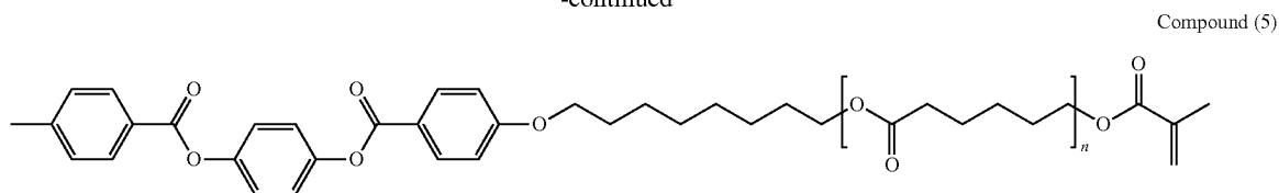
4-((4-((8-((6-(methacryloyloxy)hexanoyl)oxy)octyl)oxy)benzoyl)oxy)phenyl 4-methylbenzoate (n = 3)
