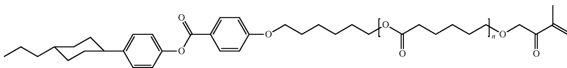
n \sim 1 1-(5-(6-(4-(trans-4-propylcyclohexyl)phenoxy)hexyloxy)-5-oxopentyloxy)-2-methylprop-2-en-1-one
