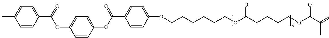
n \sim 8.7 1-(5-(5-(5-(5-(5-(5-(5-(6-(4-(4-methylbenzoyloxy)phenoxy)hexyloxy)-5-oxopentyloxy)-5-oxopentyloxy)-5-oxopentyloxy)-5-oxopentyloxy)-5-oxopentyloxy)-5-oxopentyloxy)-5-oxopentyloxy)-2-methylprop-2-en-1-one
