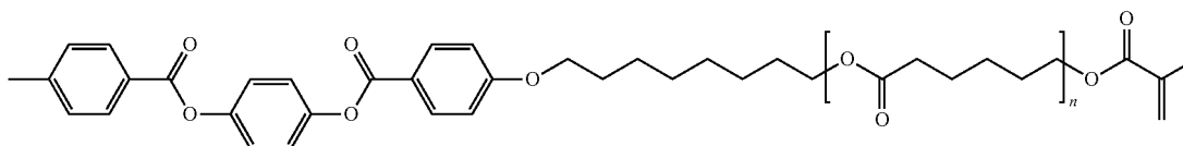
4-(((4-((8-((6-(methacryloyloxy)hexanoyl)oxy)octyl)oxy)benzoyl)oxy)phenyl 4-methylbenzoate (n = 8)
