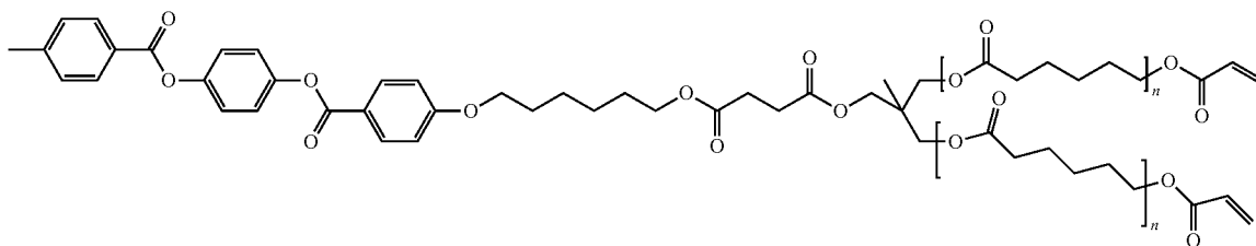
n \sim 1 1-[3-(6-(acryloyloxy)hexanoyloxy)-2-((6-(acryloyloxy)hexanoyloxy)methyl)-2-methylpropyloxy]-4-[6-(4-((4-(4-methylbenzoyloxy)phenoxy)carbonyl)phenoxy)hexyloxy]-butan-1,4-dione
