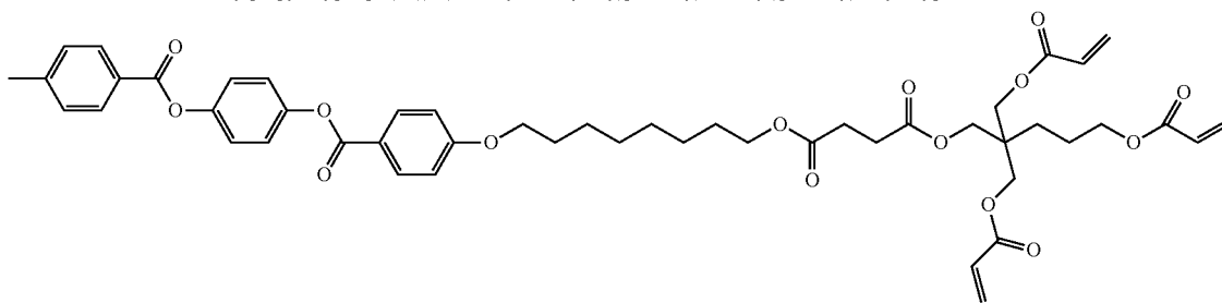
1-[3-(acryloyloxy)-2,2-bis(acryloyloxymethyl)propyloxy]-4-[8-(4-((4-(4-methylbenzoyloxy)phenoxy)carbonyl)phenoxy)octyloxy]-butan-1,4-dione
