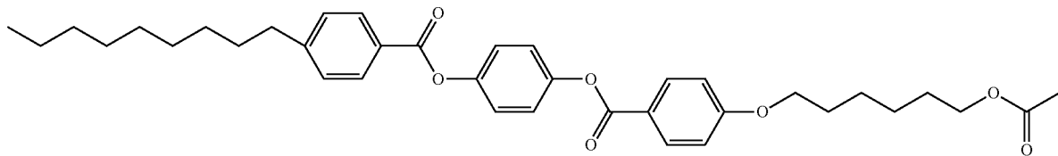
1-(3-(4-(3-(4-(6-(4(4-(6-methacryloyloxyhexyloxy)benzoyloxy)phenyl)benzoyloxy)hexyloxy)-4-oxobutoyloxy)propyloxy)benzoyloxy)propyloxy}-4-((6-(4(4-(6-methacryloyloxyhexyloxy)benzoyloxy)phenyl)benzoyloxy)hexyloxy))-butane-1,4-dione
