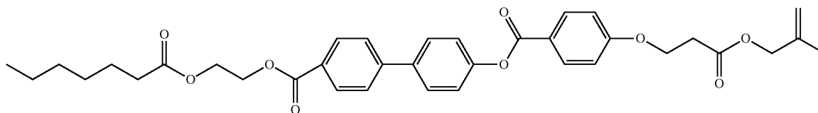
1,12-bis(2-(4-(4-(4-(3-(methacryloyloxy)propyloxy)benzoyloxy)phenyl)benzoyloxy)ethyloxy) dodecyl-1,12-dione
