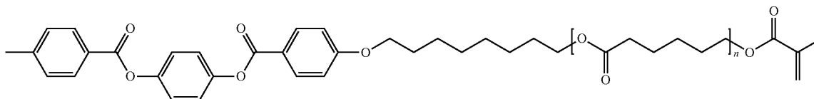
n \sim 7 1-(6-(6-(6-(6-(6-(6-(8-(4-(4-methylbenzoyloxy)phenoxy)octyloxy)-6-oxohexyloxy)-6-oxohexyloxy)-6-oxohexyloxy)-6-oxohexyloxy)-6-oxohexyloxy)-6-oxohexyloxy)-2-methylprop-2-en-1-one
