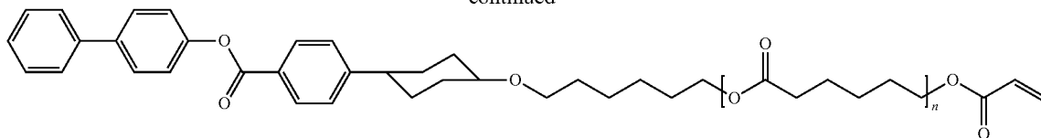
n \sim 2 1-(6-(6-(6-(trans-4-(4-phenylphenoxy)carbonyl)phenyl)cyclohexyloxy)hexyloxy)-6-oxohexyloxy)-6-oxohexyloxy)prop-2-en-1-one
