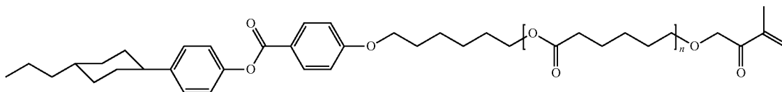
n \sim 6.4 1-(5-(5-(5-(5-(5-(5-(6-(4-(4-(trans-4-propylcyclohexyl)phenoxy)carbonyl)phenoxy)hexyloxy)-5-oxopentyl)oxy)-5-oxopentyl)oxy)-5-oxopentyl)oxy)-5-oxopentyl)oxy)-2-methylprop-2-en-1-one
