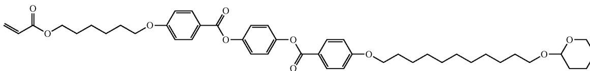
1-(11-(4-(4-(4-(6-(11-(tetrahydro-2H-pyran-2-yloxy)undecanyloxy)benzoyloxy)phenoxy)carbonyl)phenoxy)hexyloxy)prop-2-en-1-one
