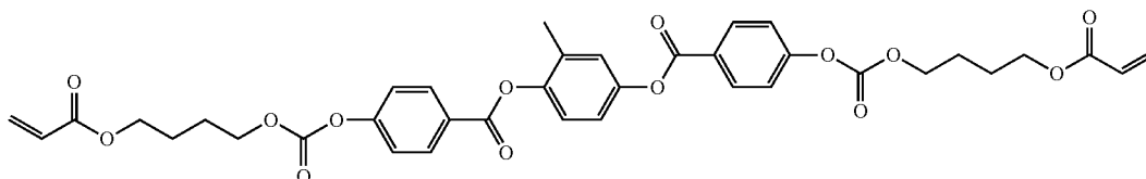
2-methyl-1,4-phenylene bis(4-(((4-(acryloyloxy)butoxy)carbonyl)oxy)benzoate)
