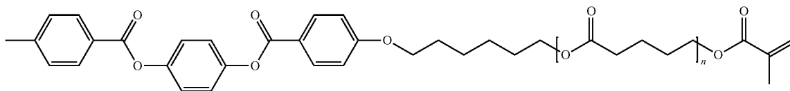
n \sim 8.1 1-(5-(5-(5-(5-(5-(5-(5-(6-(4-(4-methylbenzoyloxy)phenoxy)hexyloxy)-5-oxopentyloxy)-5-oxopentyloxy)-5-oxopentyloxy)-5-oxopentyloxy)-5-oxopentyloxy)-5-oxopentyloxy)-2-methylprop-2-en-1-one
