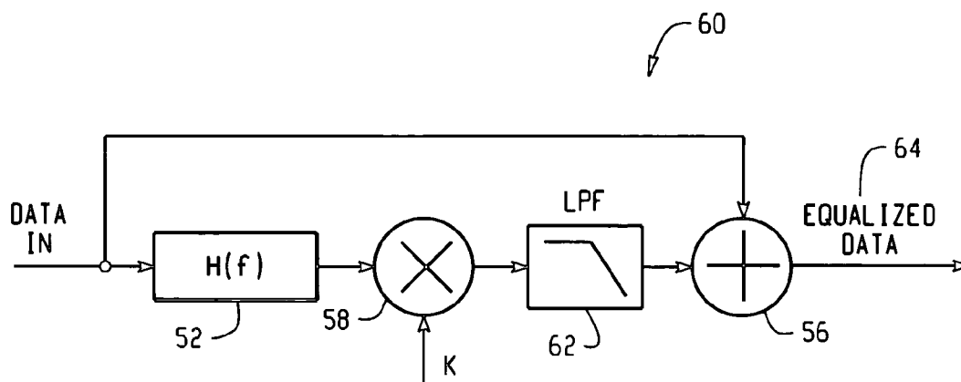
Fig. 5 RELATED ART
