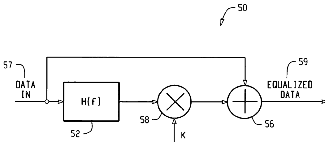
Fig. 4 RELATED ART
