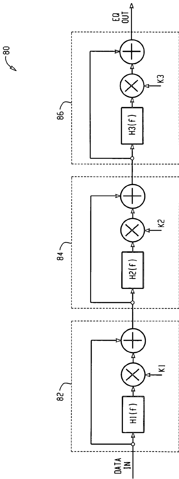
Fig. 7 RELATED ART
