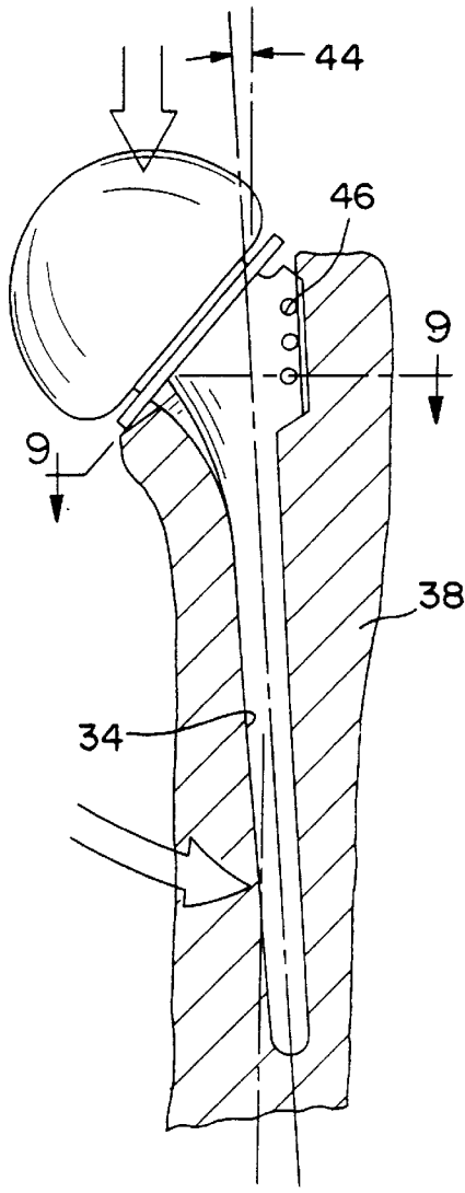
FIG. 8 PRIOR ART
