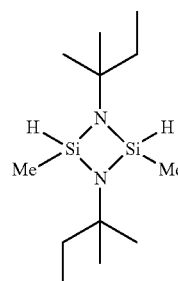
1,3-bis(tert-amyly)-2,4-dimethylcyclodisilazane
