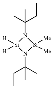
1,3-bis(tert-amyl)-2- dimethylcyclodisilazane
