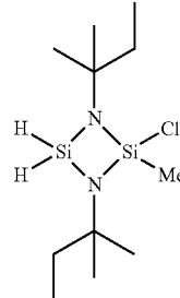
1,3-bis(tert-amyl)-2-chloro-2-methyl- cyclodisilazane
