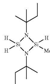
1,3-bis(tert-amyly)-2-methylcyclodisilazane
