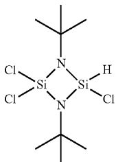
1,3-bis(tert-butyl)-2,2,4-trichloro- cyclodisilazane
