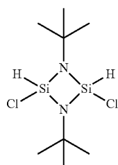
1,3-bis(tert-butyl)-2,4-dichlorocyclodisilazane
