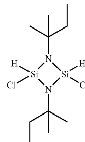
1,3-bis(tert-amyly)-2,4-dichloro-cyclodisilazane
