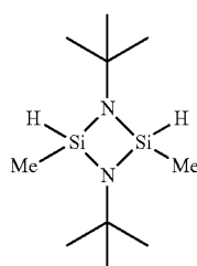
1,3-bis(tert-butyl)-2,4-dimethylcyclodisilazane
