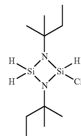
1,3-bis(tert-amyly)-2-chloro-cyclodisilazane
