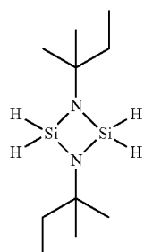
1,3-bis(tert-amyly)cyclodisilazane
