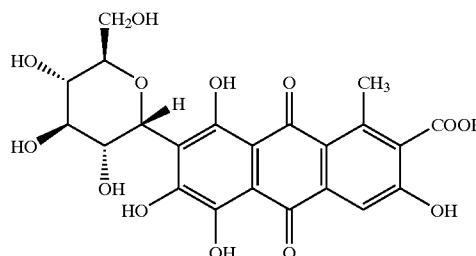
Carminic Acid
