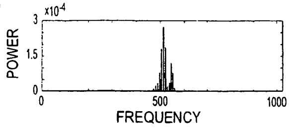
IQ SIGNAL SPECTRUM OF CREATED CONTINUOUS WAVE
