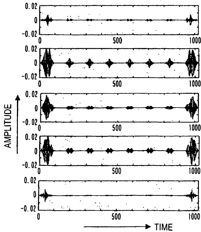
CONTINUOUS WAVE SYNTHESIZED IN INVERSE FFT/SCALING PROCESS
