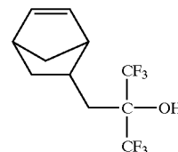
Norbornene-5-(1,1,1-trifluoro-2-trifluoromethyl)propan-2-ol (NB-HFOH)
