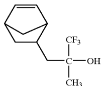
Norbornene-5-(2-trifluoromethyl)propan-2-ol (NB-TFOH)
