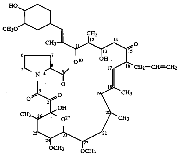
16-Allyl-1,13-dihydroxy-11-[2-(4-hydroxy-3-methoxycyclohexyl)-1-methylvinyl]-22,24-dimethoxy-12,18,20,26-tetramethyl-10,27-dioxo-4-azatricyclo-[21.3.1.0 4,8 ]heptacos-17-ene-2,3,9,15-tetraone
