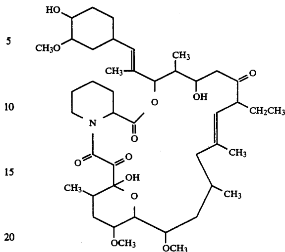
17-Ethyl-1,14-dihydroxy-12-[2-(4-hydroxy-3-methoxycyclohexyl)-1-methylvinyl]-23,25-dimethoxy-13,19,21,27-tetramethyl-11,28-dioxa-4-azatricyclo-[22.3.1.0 4,8 ]octacos-18-ene-2,3,10,16-tetraone
