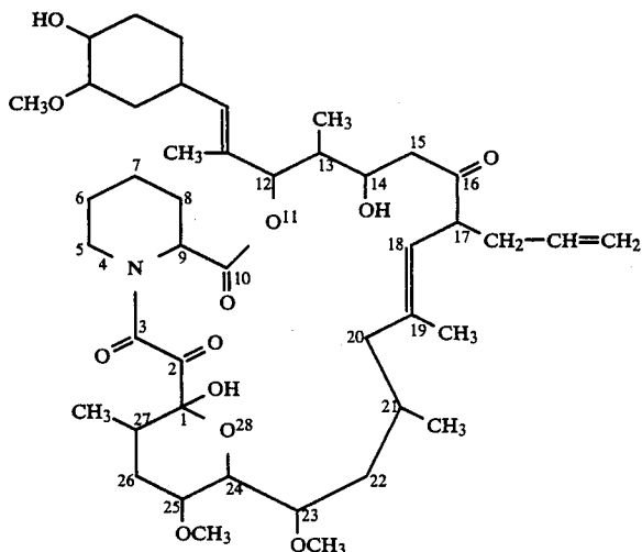
17-Allyl-1,14-dihydroxy-12-[2-(4-hydroxy-3-methoxycyclohexyl)-1-methylvinyl]-23,25-dimethoxy-13,19,21,27-tetramethyl-11,28-dioxo-4-azatricyclo[22.3.1.0 4,9 ]octacos-18-ene-2,3,10,16-tetraone
