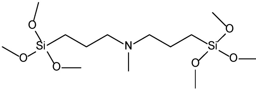
-N-Methyl-3-(triethoxysilyl)-N-[3-(triethoxysilyl)propyl]-1-propanamin
