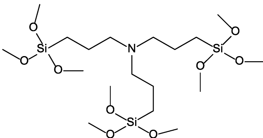
- 3-(Triethoxysilyl)-N,N-bis[3-(triethoxysilyl)propyl]-1-propanamin
