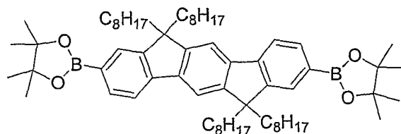
Alkyl-indenofluorene
