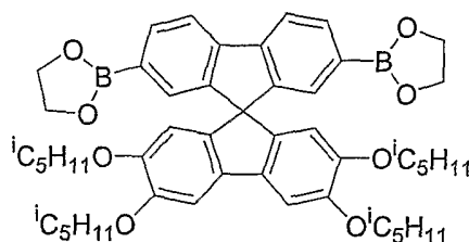
Spirofluorene
