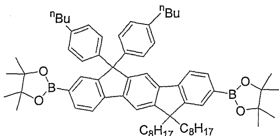
Alkyl-aryl-indenofluorene
