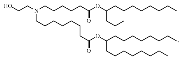
(Compound 78)
