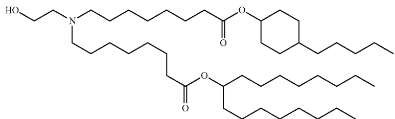
(Compound 67)
