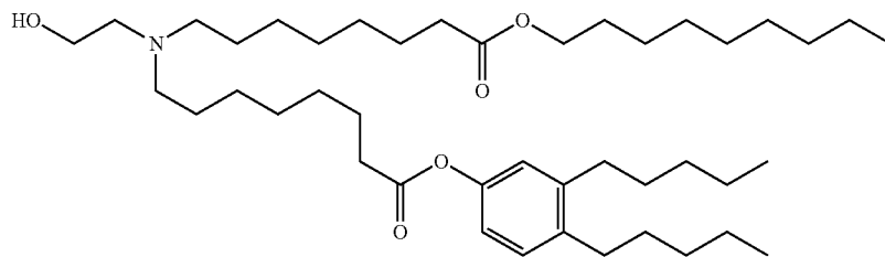
3,4-Dipentylphenyl 8-((2-hydroxyethyl)(8-nonyloxy)-8-oxooctyl)amino)octanoate
