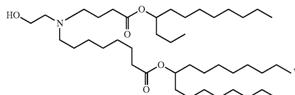
(Compound 76)
