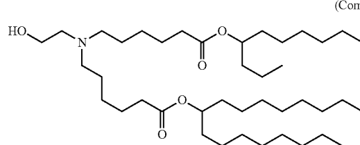
(Compound 93)
