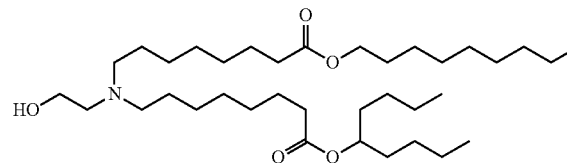
Chemical Formula: C 36 H 71 NO 5 Molecular Weight: 597.97
