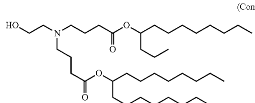
(Compound 92)
