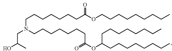
(Compound 10)
