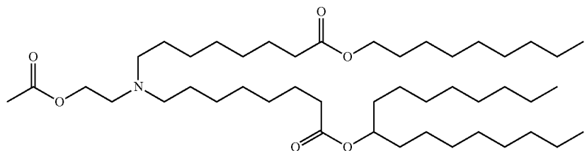
(Compound 10)
