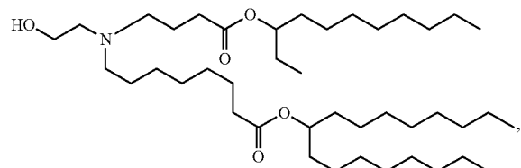
(Compound 74)
