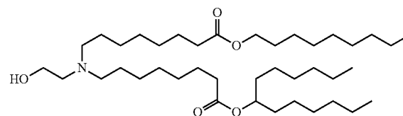
Chemical Formula: C 40 H 79 NO 5 Molecular Weight: 654.07
