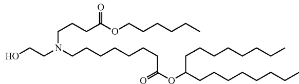
Chemical Formula: C 37 H 73 NO 5 Molecular Weight: 611.99
