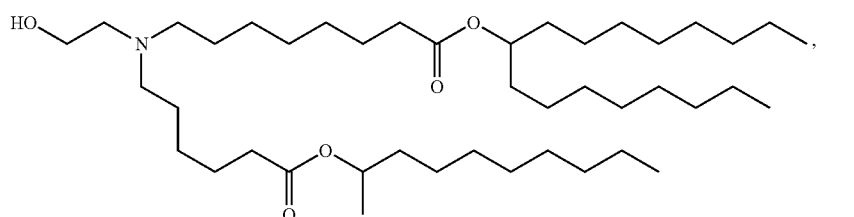
(Compound 123)
