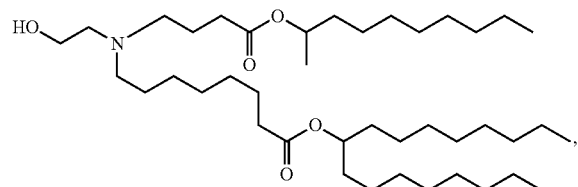
(Compound 72)
