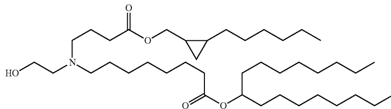
Chemical Formula : C 41 H 79 NO 5 Molecular Weight: 666.09
