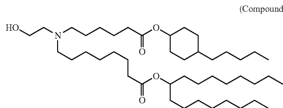
(Compound 67)
