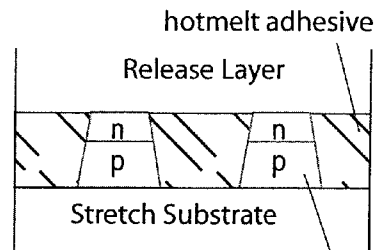
Figure 83(a) embedded LED chips
