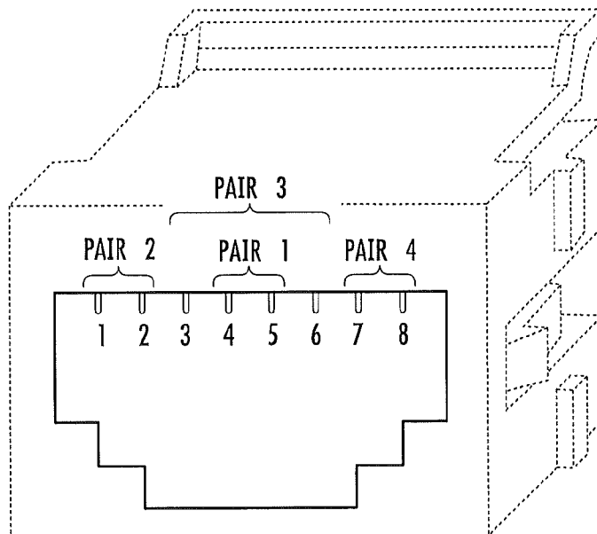
FIG. 2 (PRIOR ART)
