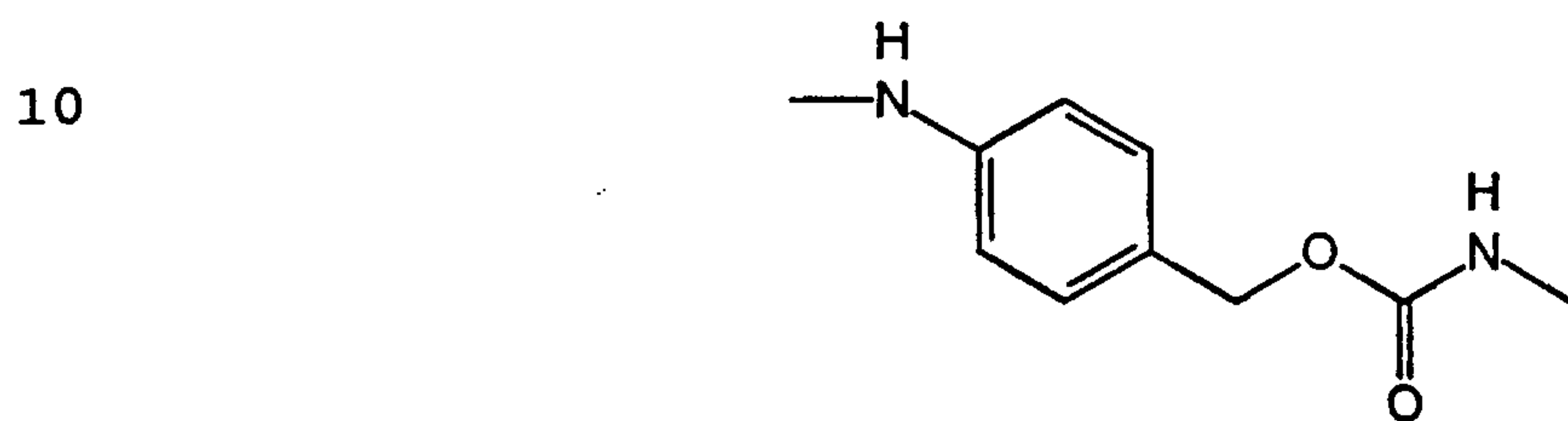
15 Formula (IIIa)
