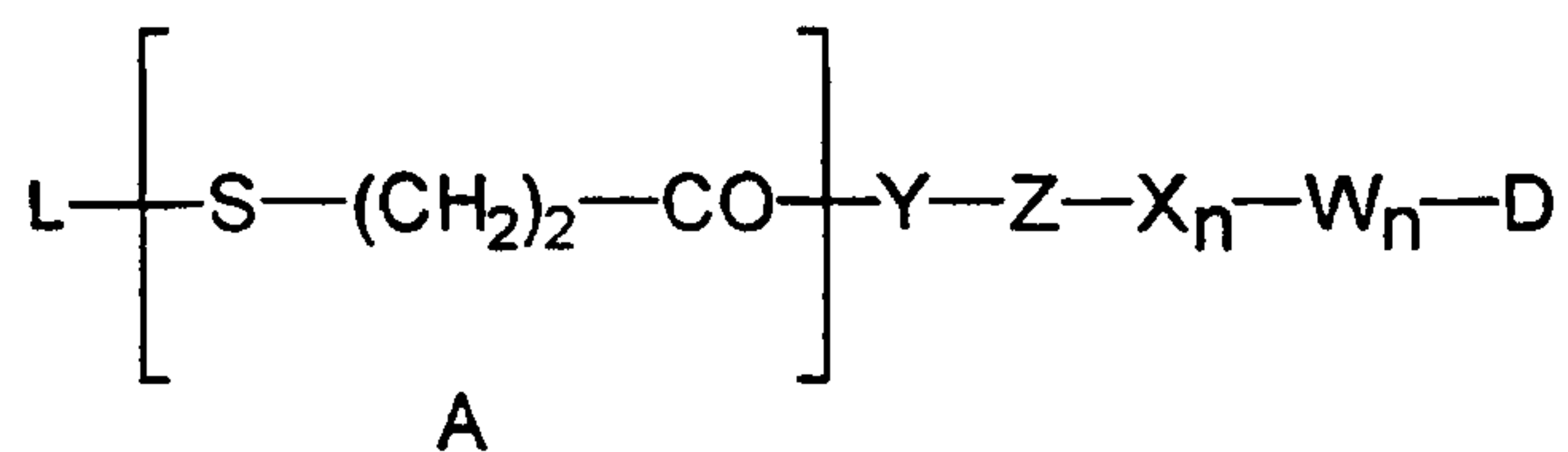
Formula (Xa)
