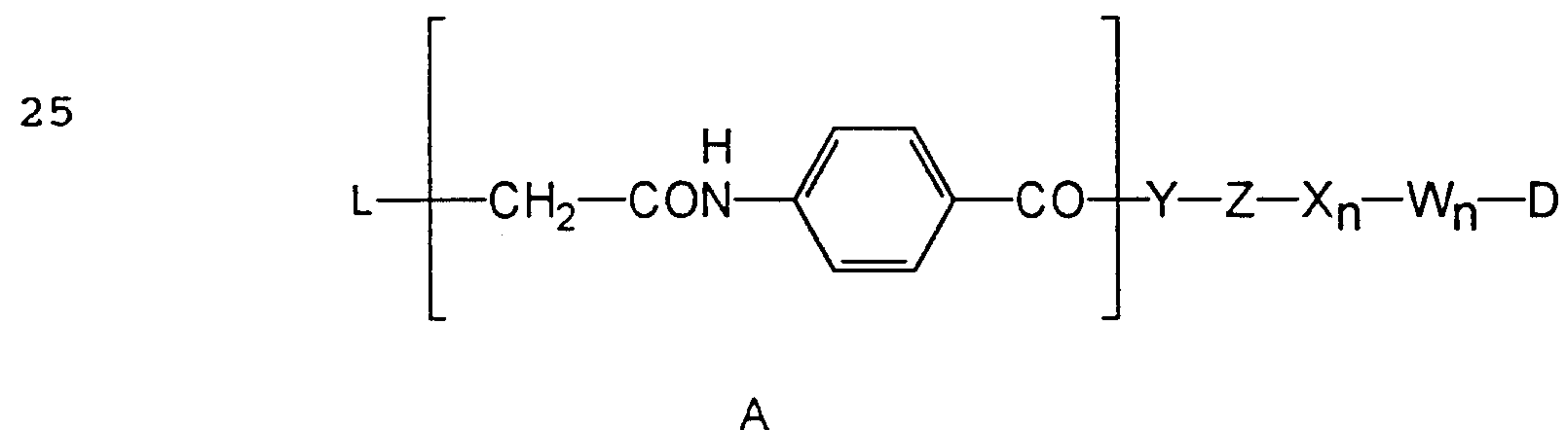
Formula (IXe)
