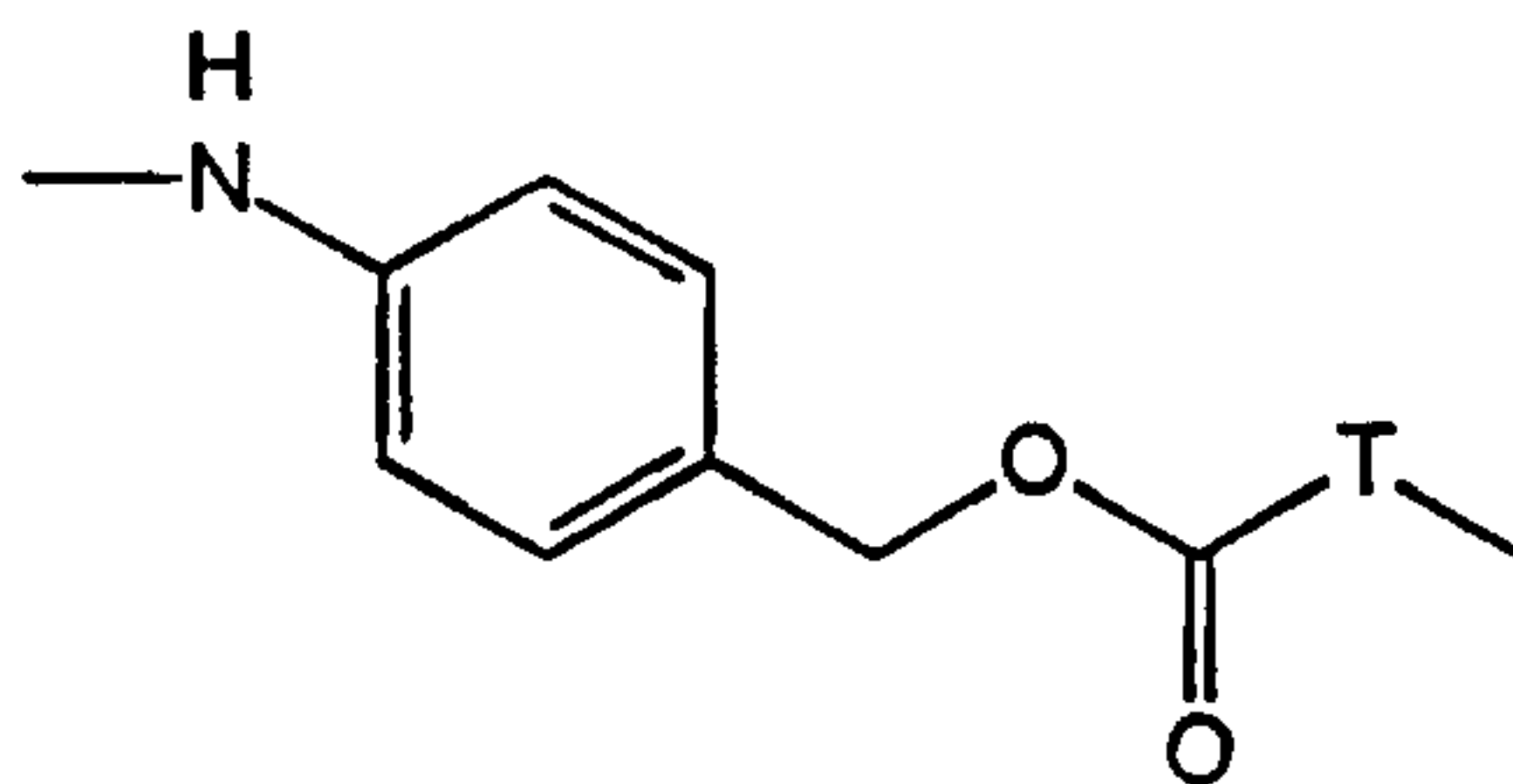
Formula (III)
