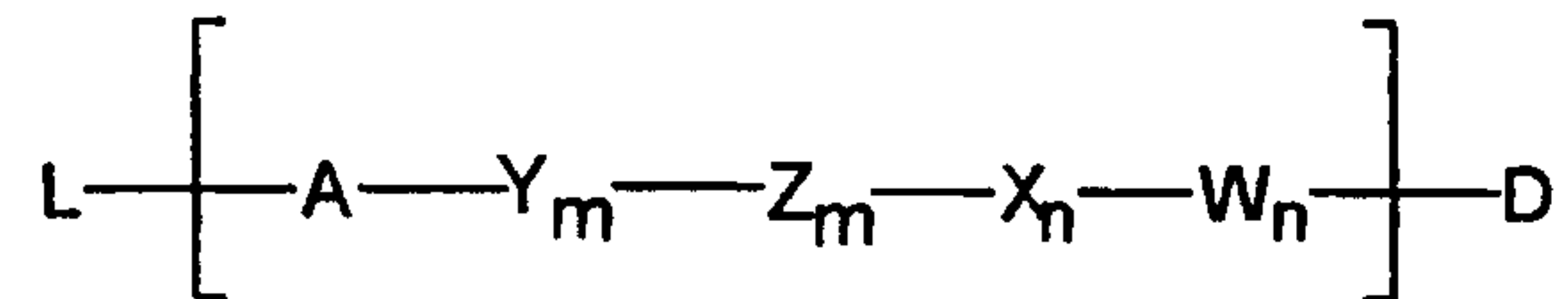
Formula (I)
