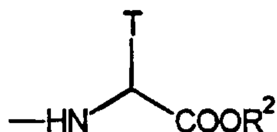
Formula (V)
