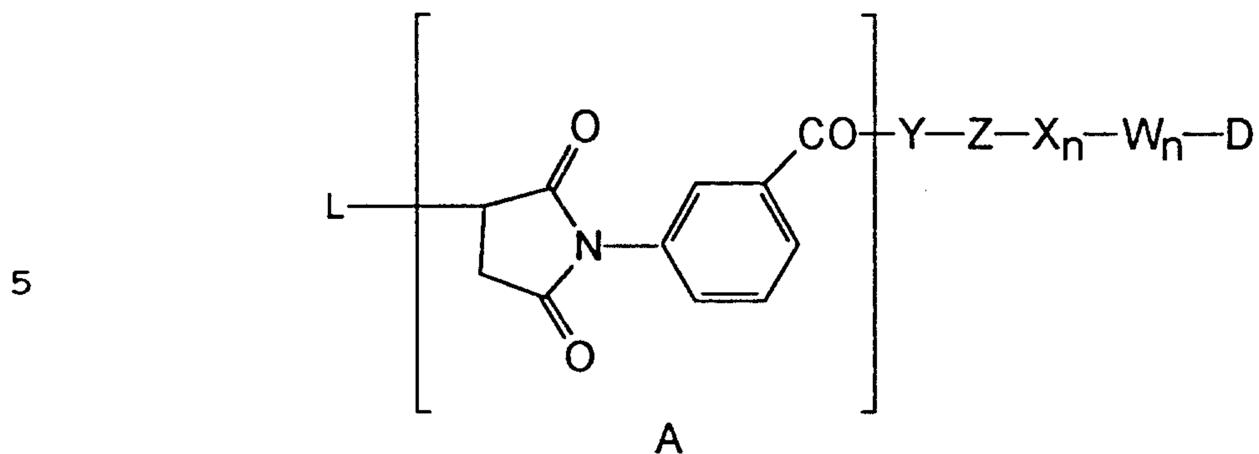
Formula (IXc)
