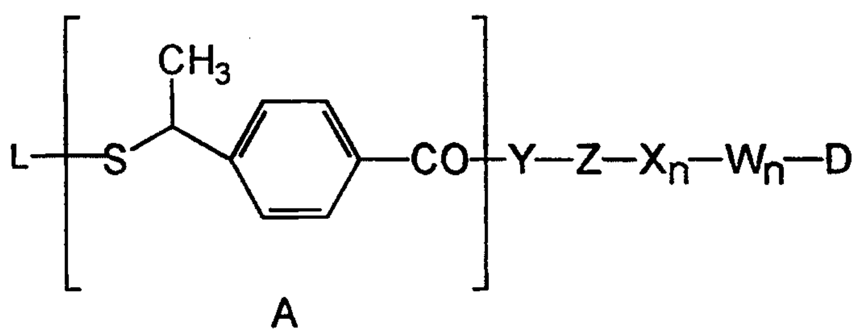
Formula (Xb)
