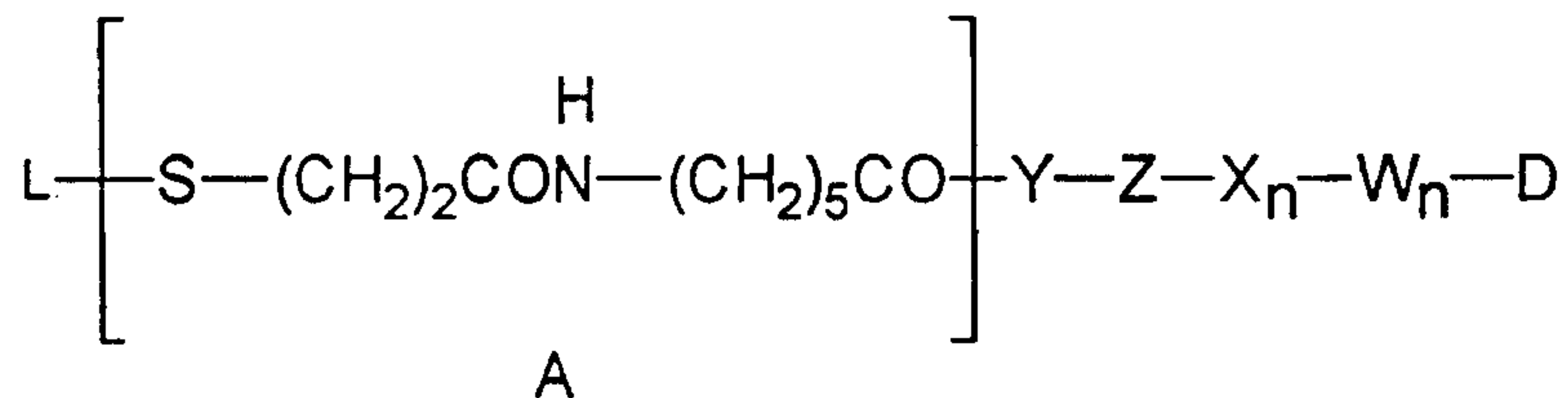
Formula (Xc)
