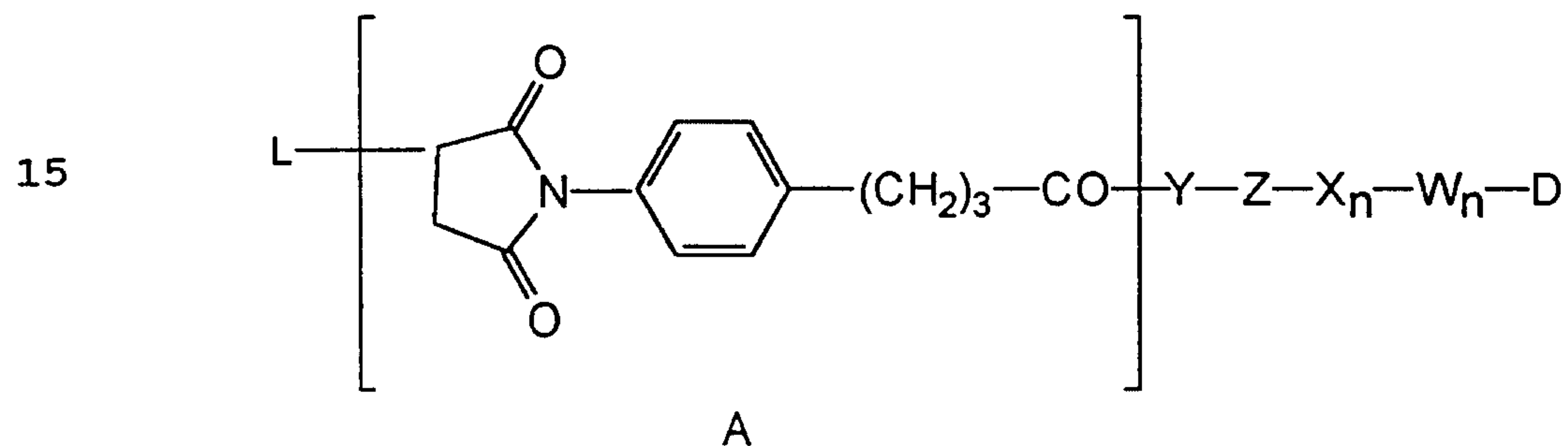
Formula (IXd)
