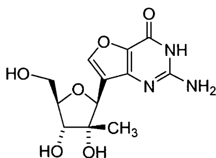
2-amino-7-(2-C-methyl- \beta -D-ribofuranosyl)-furo[3,2- d ]pyrimidin-4(3 H )-one
