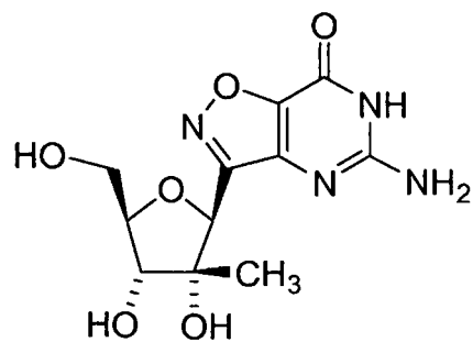
5-amino-3-(2-C-methyl- \beta -D-ribofuranosyl)-isoxazolo-[4,5- d ]pyrimidin-7(6 H )-one
