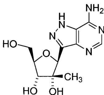
7-Amino-3-(2-C-methyl-β-D-ribofuranosyl)-1H-pyrazolo[4,3-d]pyrimidine
