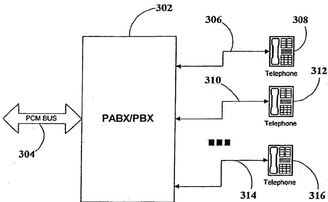
FIG. 3. (PRIOR ART)
