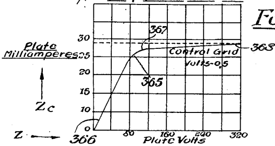
Pentode Amplifier CHARACTERISTICS Type 6AC7 screen Volts 150
