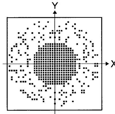
ARRANGEMENT PATTERN OF ELEMENTS FOR TRANSMISSION/RECEPTION
