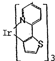
Compound 7
