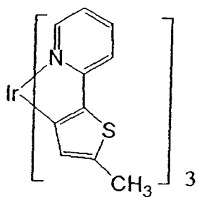
Compound 14
