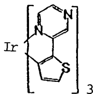
Compound 8
