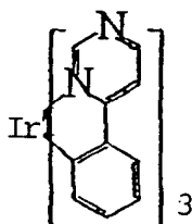
Compound 3
