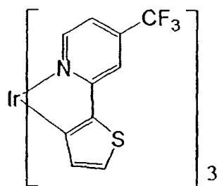
Compound 15
