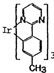
Compound 4
