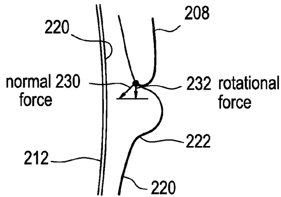
FIG. 2 PRIOR ART
