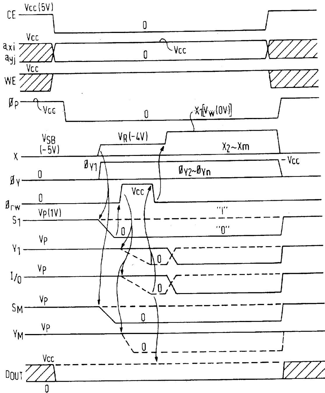
WRITE OPERATION
