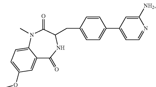
(compound 3) 40
