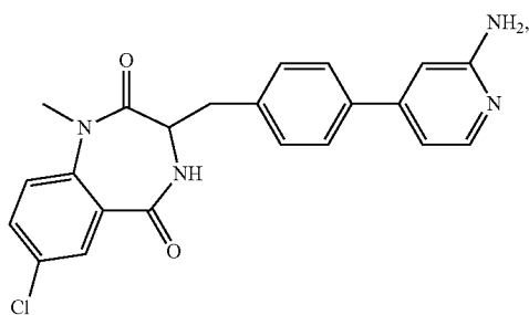
(compound 3)
