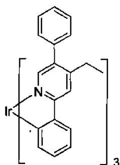
Compound 22
