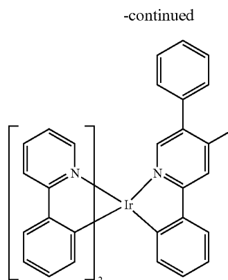
Compound 12
