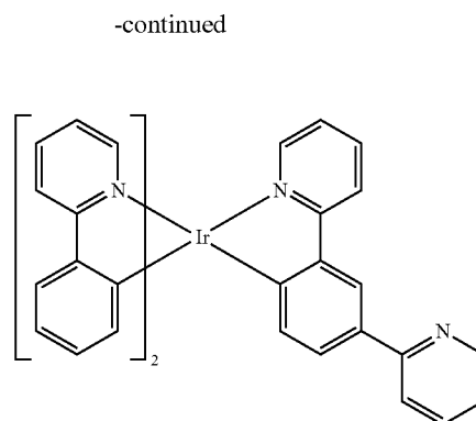
Compound 4
