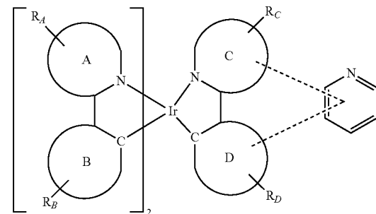
Compound 3
