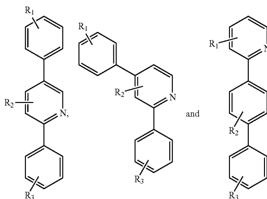
Compound 14
