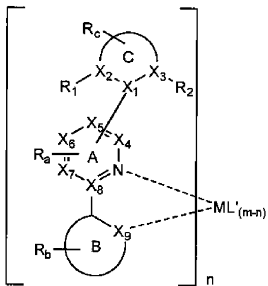
Formula II
