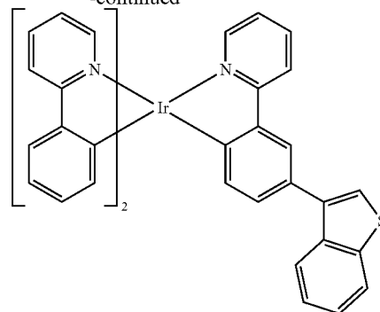
Compound 6
