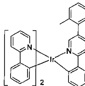
Compound 25
