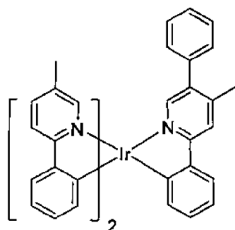
Compound 31
