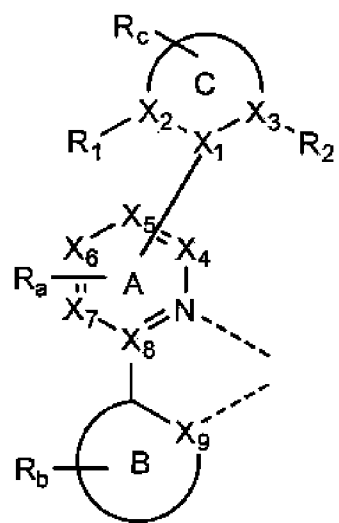
Formula I
