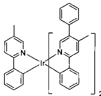
Compound 34
