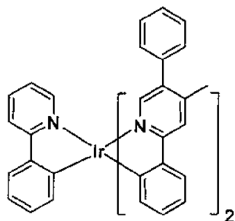
Compound 29
