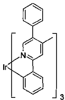
Compound 21
