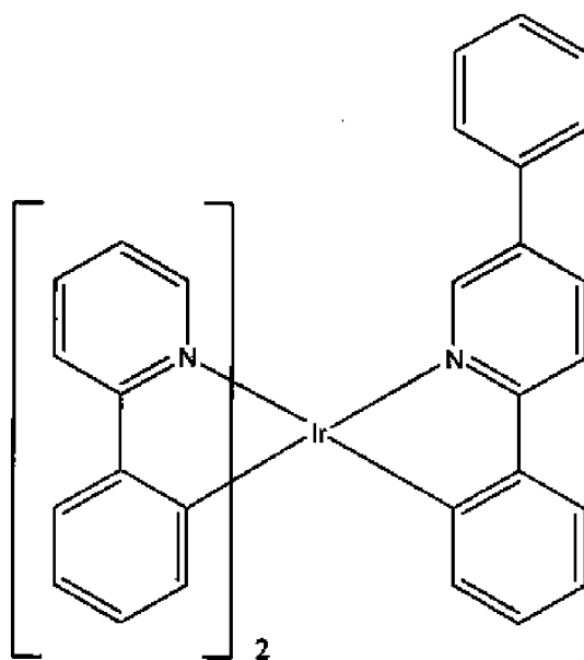
Compound 2
