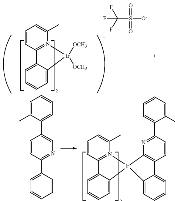
Compound 26
