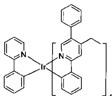
Compound 30
