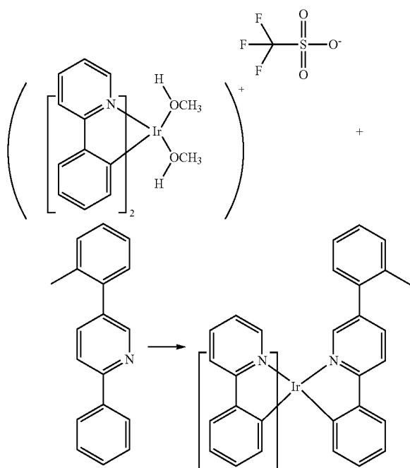
Compound 25
