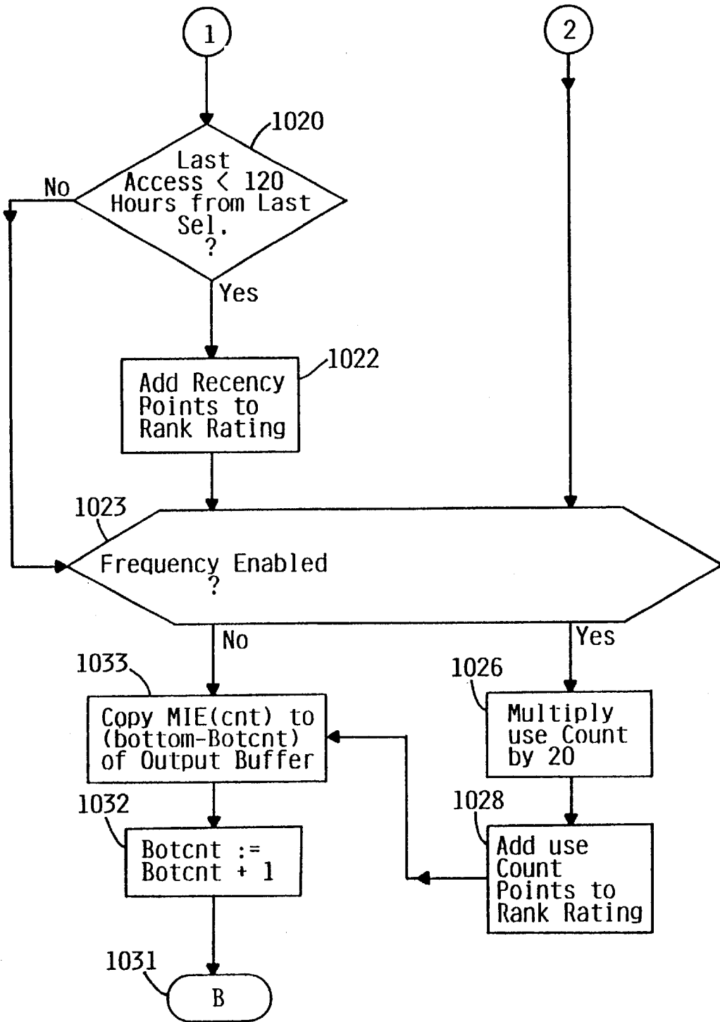
Menu Adjuster 255 - Automatic Ranking
