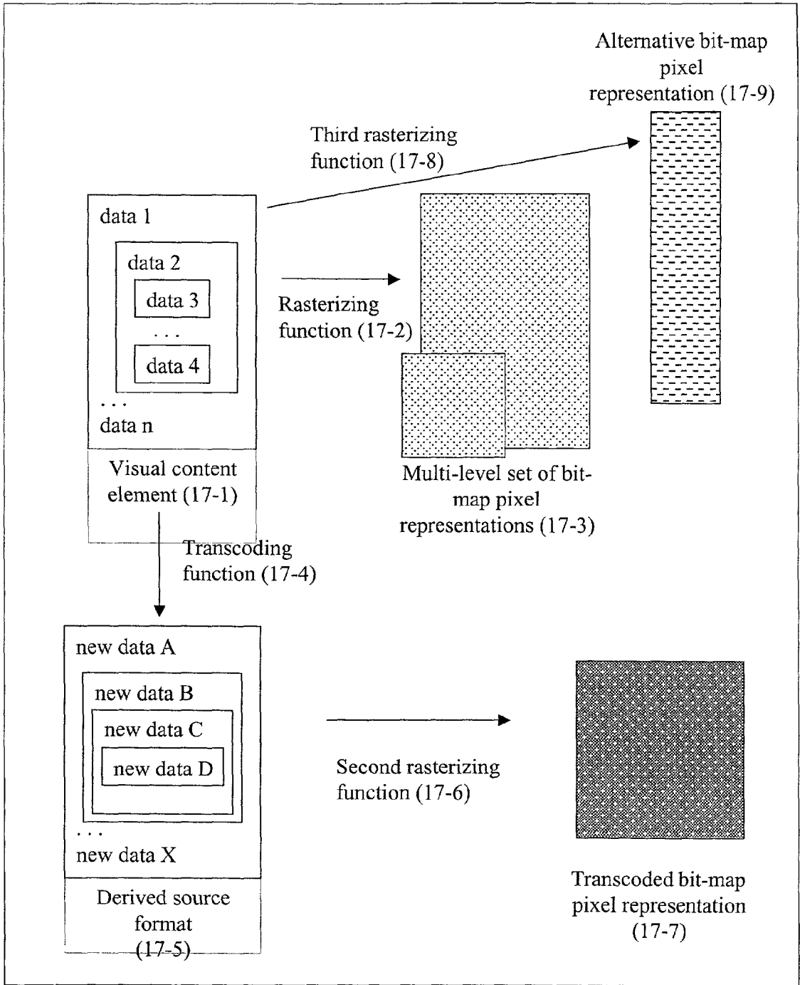
Figure 17: Multi-Modal Set of Representations
