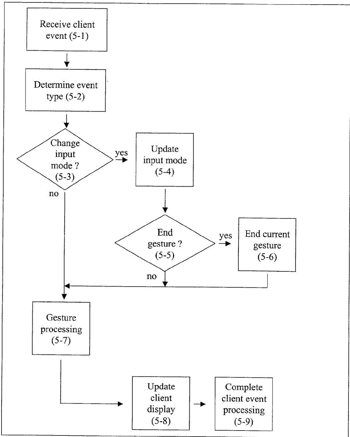
Figure 5: Client Processing of Events
