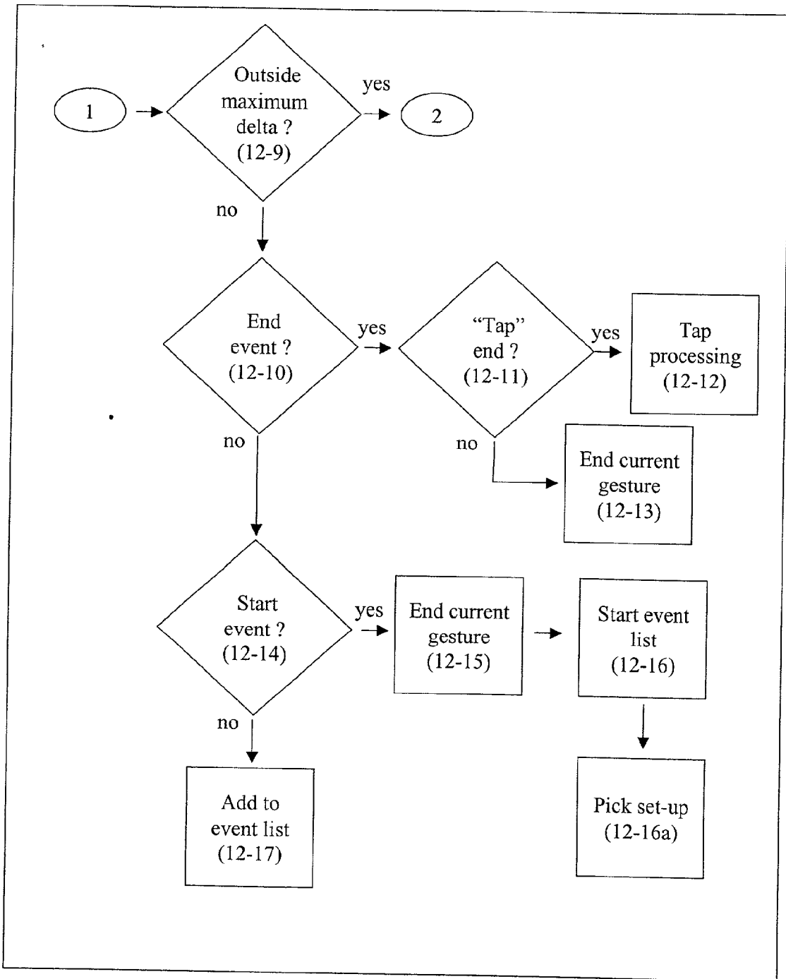
Figure 12 (continued): Selection Mode Gesture Processing P. 2 of 7
