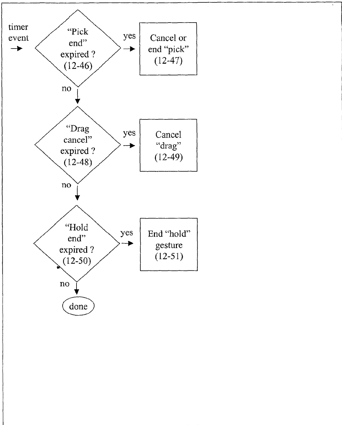
Figure 12 (continued): Selection Mode Gesture Processing P. 7 of 7
