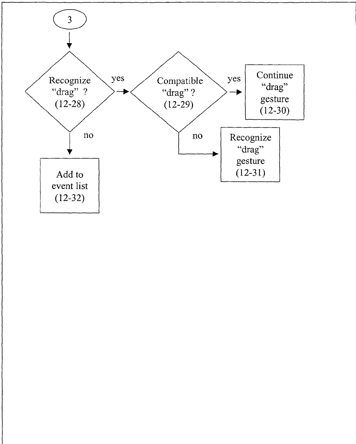
Figure 12 (continued): Selection Mode Gesture Processing P. 4 of 7
