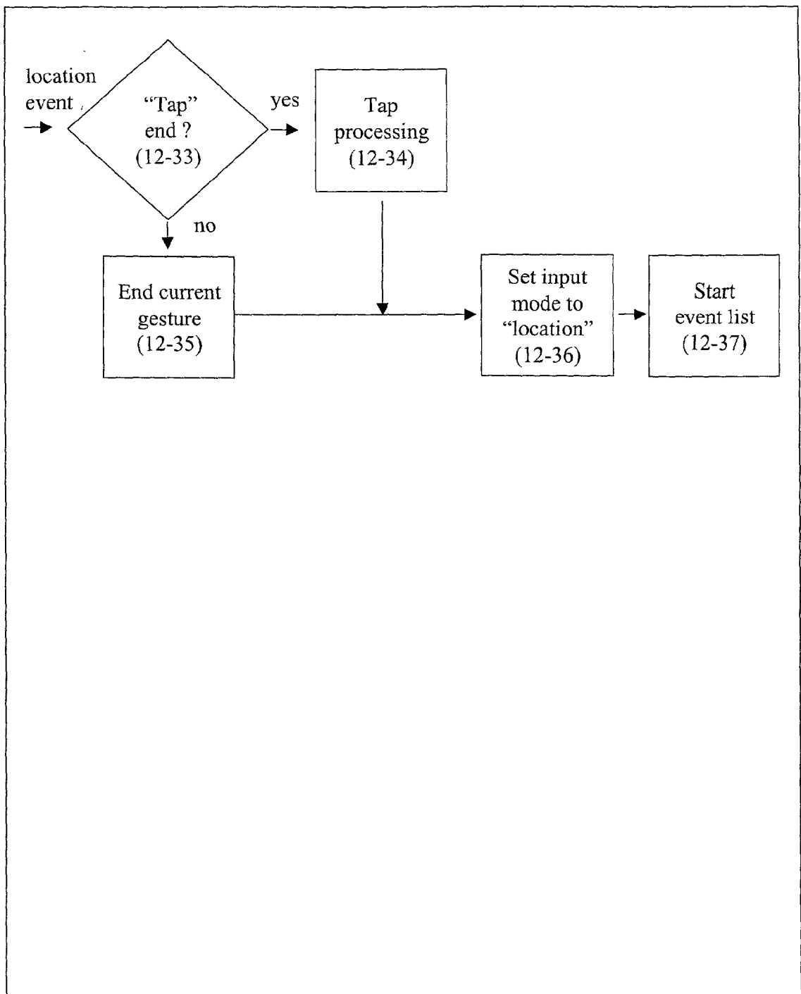
Figure 12 (continued): Selection Mode Gesture Processing P. 5 of 7
