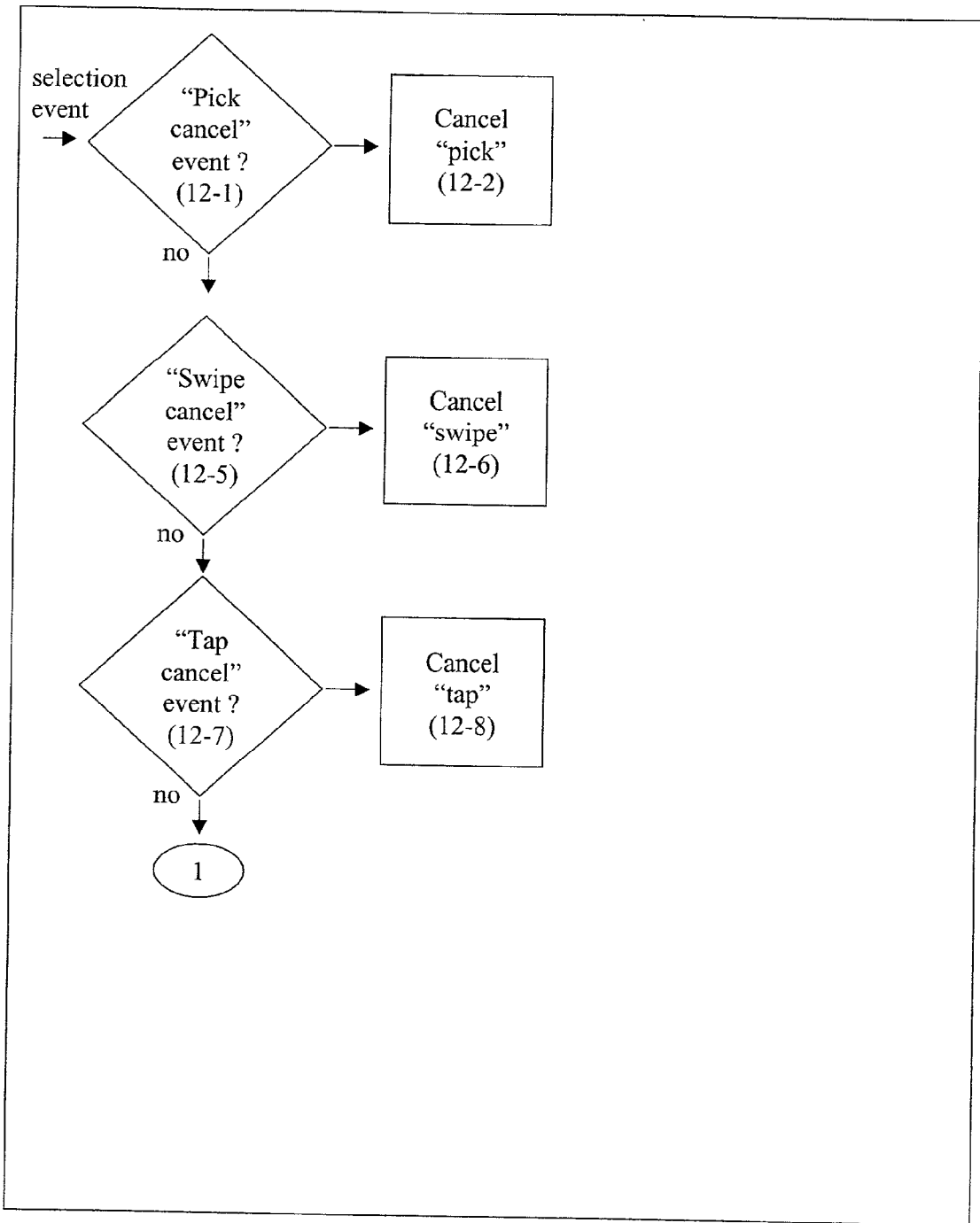
Figure 12: Selection Mode Gesture Processing P. 1 of 7
