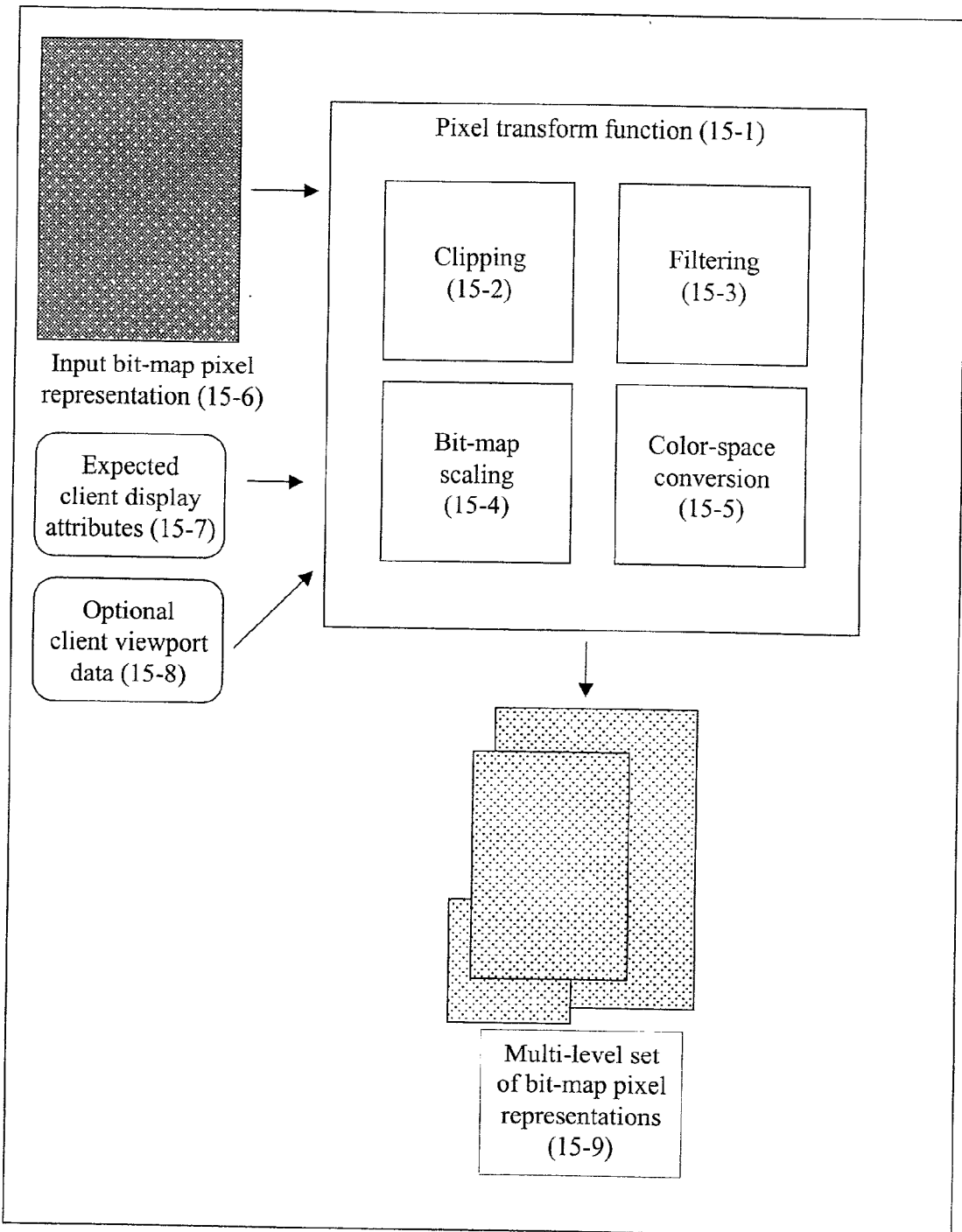
Figure 15: Pixel transform function
