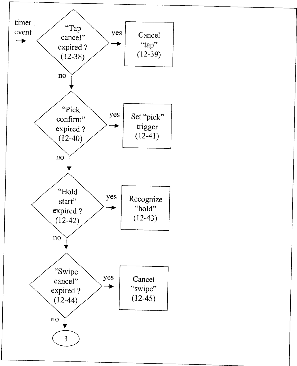
Figure 12 (continued): Selection Mode Gesture Processing P. 6 of 7
