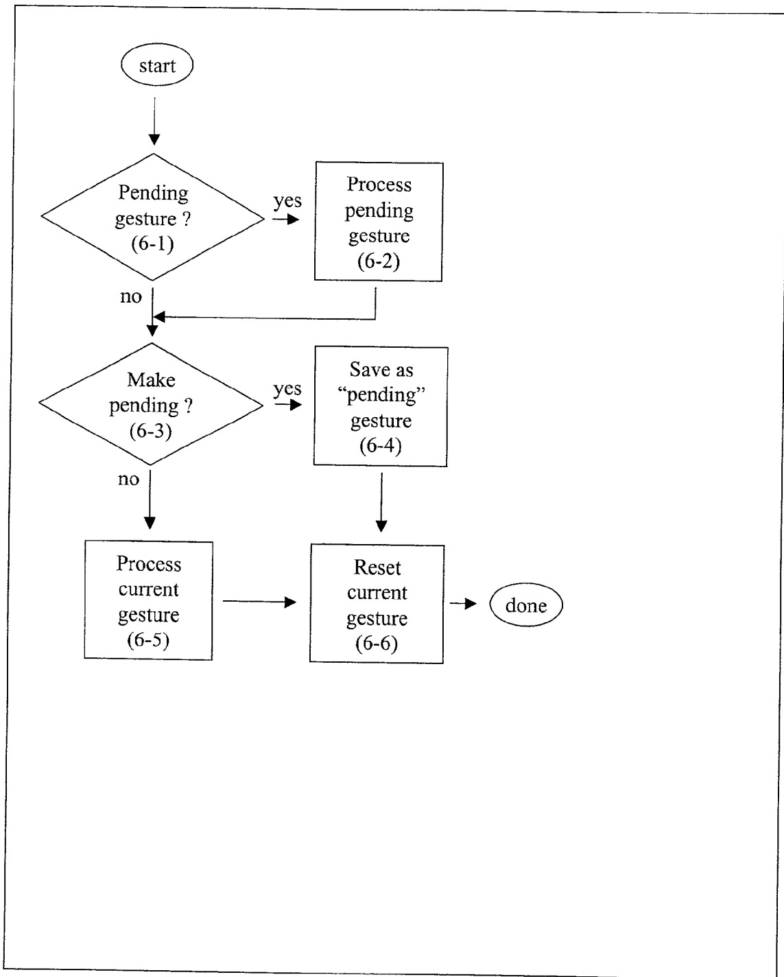
Figure 6: "End Gesture" Processing
