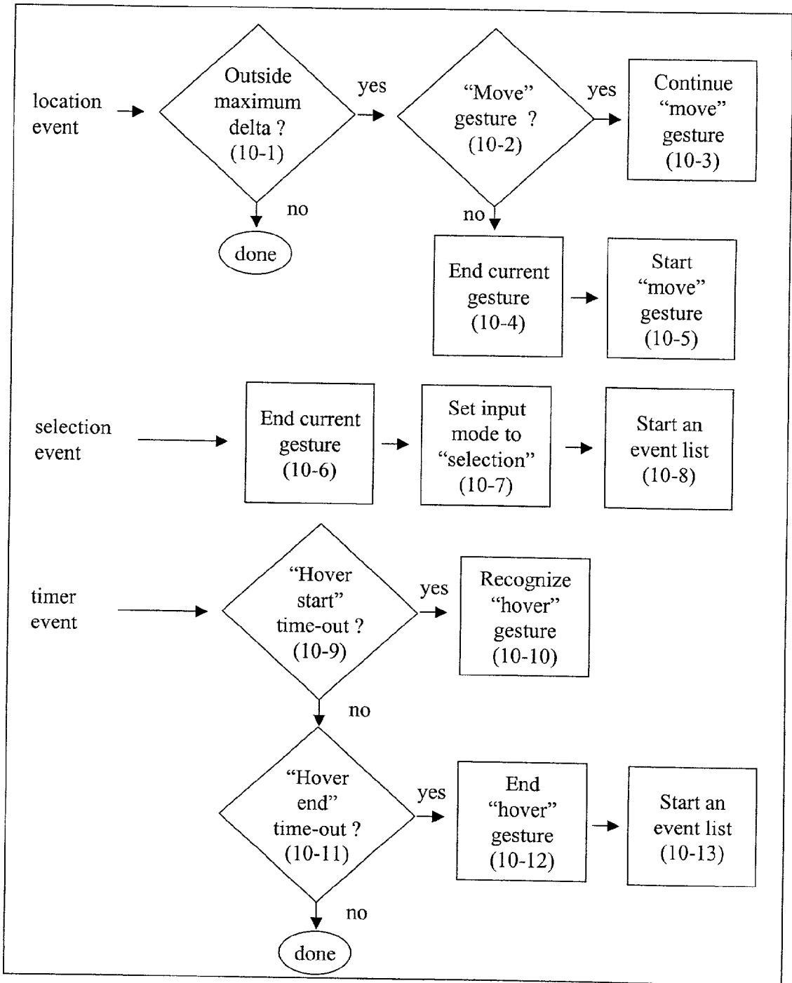
Figure 10: Location Mode Gesture Processing
