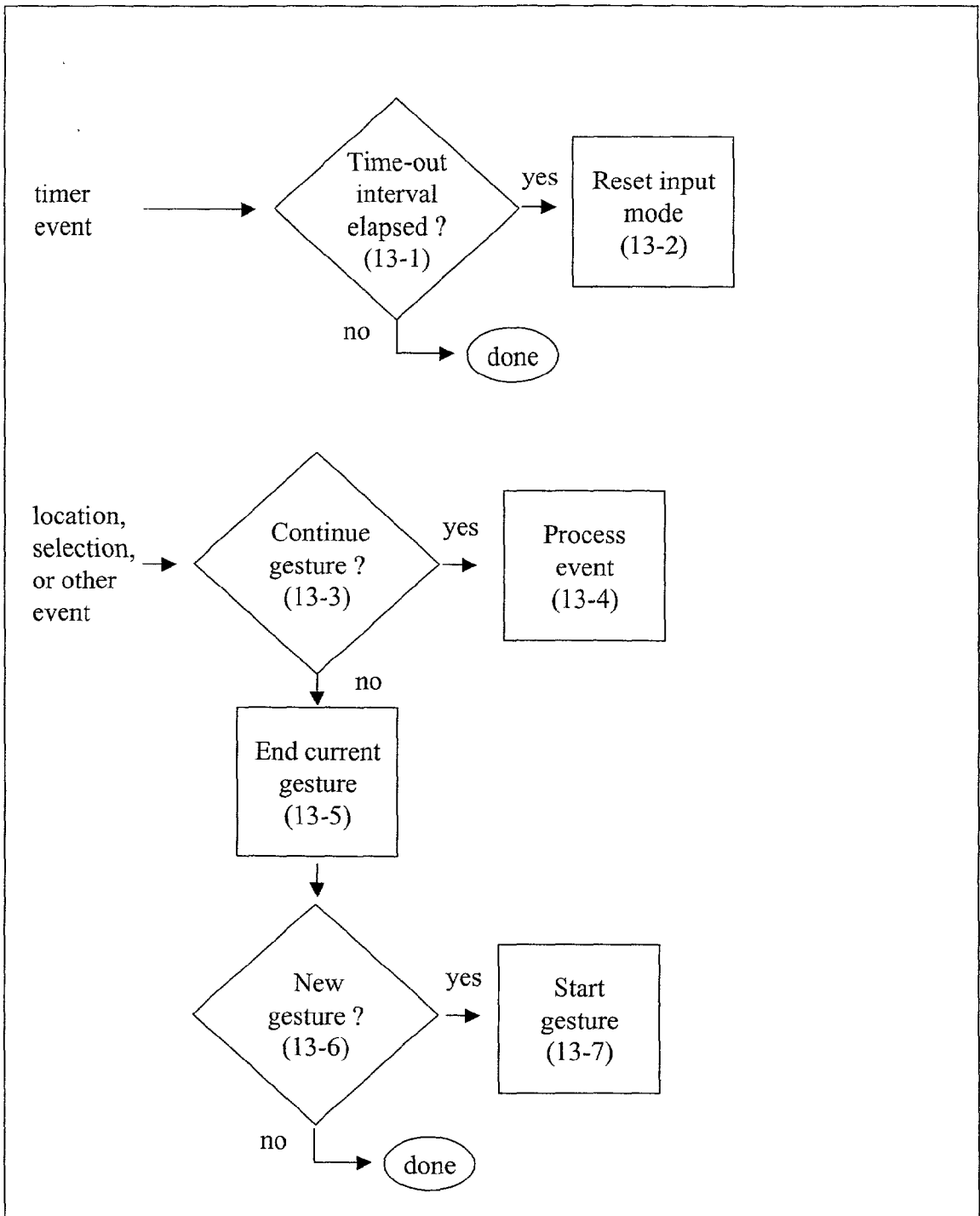
Figure 13: Special Input Mode Gesture Processing
