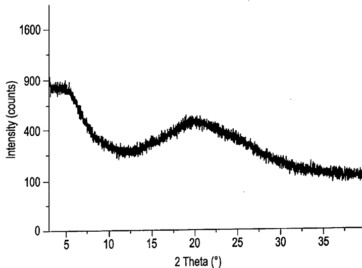
XRPD of AMG 706 Amorphous Form By Spray-drying Method
