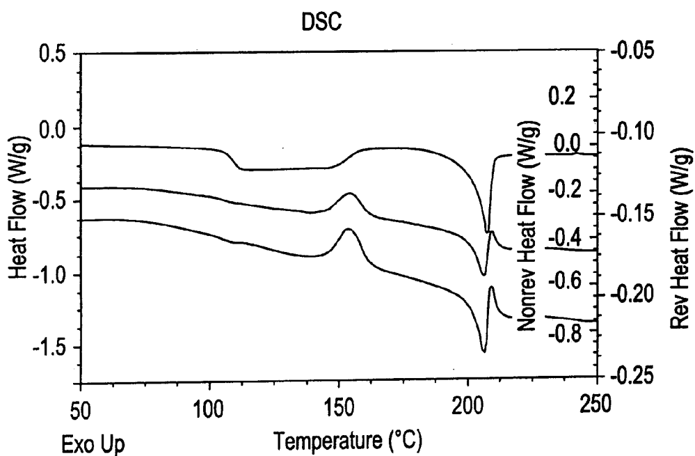
MDSC of AMG 706 Amorphous Form By Spray-drying Method
