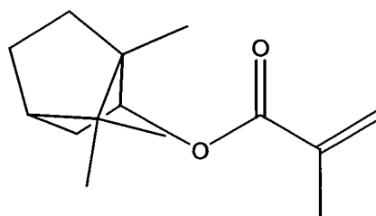
isobornyl methacrylate
