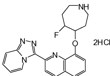
Stereoisomer #3 of 2-([1,2,4]triazolo[4,3-a]pyridin-3-yl)-8-(5-fluoroazepan-4-yloxy)quinoline dihydrochloride
