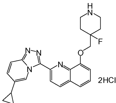
2-(6-cyclopropyl-[1,2,4]triazolo[4,3-a]pyridin-3-yl)-8-((4-fluoropiperidin-4-yl)methoxy)quinoline dihydrochloride
