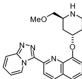
2-([1,2,4]triazolo[4,3-a]pyridin-3-yl)-8-((2S,4S)-2-(methoxymethyl)piperidin-4-yloxy)quinoline
