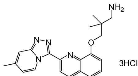
2,2-dimethyl-3-(2-(7-methyl-[1,2,4]triazolo[4,3-a]pyridin-3-yl)quinolin-8-yloxy)propan-1-amine trihydrochloride
