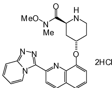
(2S,4S)-4-(2-([1,2,4]triazolo[4,3-a]pyridin-3-yl)quinolin-8-yloxy)-N-methoxy-N-methylpiperidine-2-carboxamide dihydrochloride
