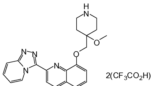
2-([1,2,4]triazolo[4,3-a]pyridin-3-yl)-8-((4-methoxypiperidin-4-yl)methoxy)quinoline bis(trifluoroacetate)
