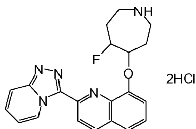
Stereoisomer #2 of 2-([1,2,4]triazolo[4,3-a]pyridin-3-yl)-8-(5-fluoroazepan-4-yloxy)quinoline dihydrochloride
