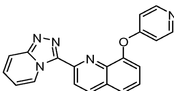
2-([1,2,4]triazolo[4,3-a]pyridin-3-yl)-8-(pyridin-4-yloxy)quinoline
