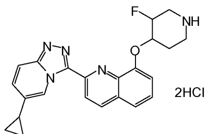
2-(6-cyclopropyl-[1,2,4]triazolo[4,3-a]pyridin-3-yl)-8-((cis)-3-fluoropiperidin-4-yl)oxyquinoline dihydrochloride
