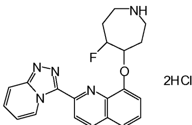
Stereoisomer #1 of 2-([1,2,4]triazolo[4,3-a]pyridin-3-yl)-8-(5-fluoroazepan-4-yloxy)quinoline dihydrochloride
