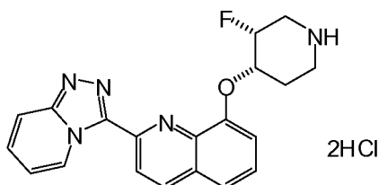
2-([1,2,4]triazolo[4,3-a]pyridin-3-yl)-8-((cis)-3-fluoropiperidin-4-yloxy)quinoline dihydrochloride
