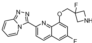
2-([1,2,4]triazolo[4,3-a]pyridin-3-yl)-6-fluoro-8-((3-fluoroazetid-3-yl)methoxy)quinoline Dihydrochloride
