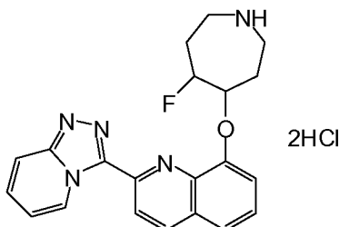
Stereoisomer #4 of 2-([1,2,4]triazolo[4,3-a]pyridin-3-yl)-8-(5-fluoroazepan-4-yloxy)quinoline dihydrochloride
