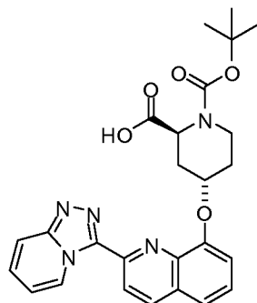
(2S,4S)-4-(2-([1,2,4]triazolo[4,3- a ]pyridin-3-yl)quinolin-8-yloxy)-1-(tert-butoxycarbonyl)piperidine-2-carboxylic acid
