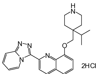
2-([1,2,4]triazolo[4,3-a]pyridin-3-yl)-8-((4-isopropylpiperidin-4-yl)methoxy)quinoline dihydrochloride
