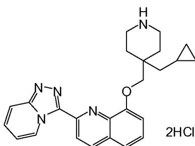
2-([1,2,4]triazolo[4,3-a]pyridin-3-yl)-8-((4-(cyclopropylmethyl)piperidin-4-yl)methoxy)quinoline dihydrochloride
