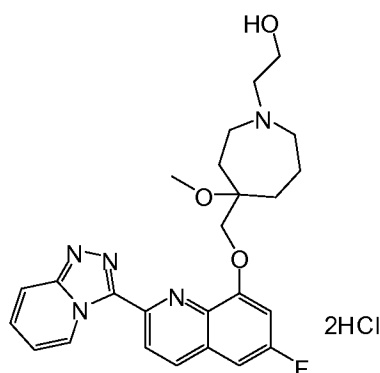
2-((4-((2-([1,2,4]triazolo[4,3-a]pyridin-3-yl)-6-fluoroquinolin-8-yloxy)methyl)-4-methoxyazepan-1-yl)ethanol) dihydrochloride
