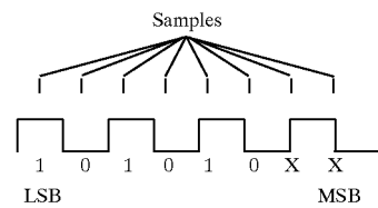
Late Sampling of Genlock Waveform
