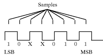
Early Sampling of Genlock Waveform
