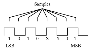
Nominal Sampling of Genlock Waveform
