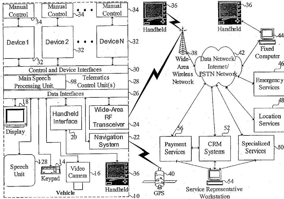
First Embodiment System Block Diagram
