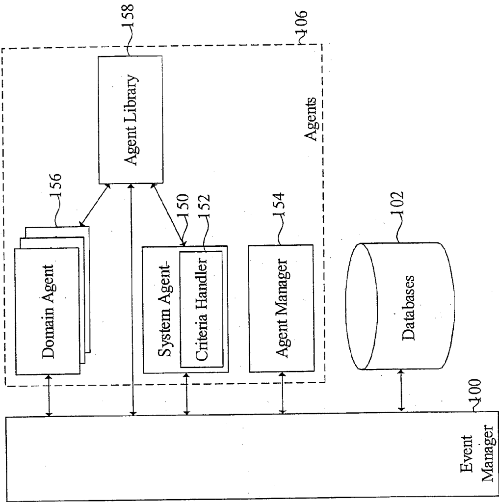
Figure 6. Agent Architecture
