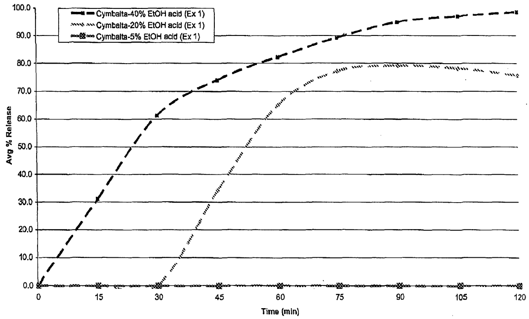
Cymbalta in 5%, 20%, 40% Ethanolic Acid (USP I)
