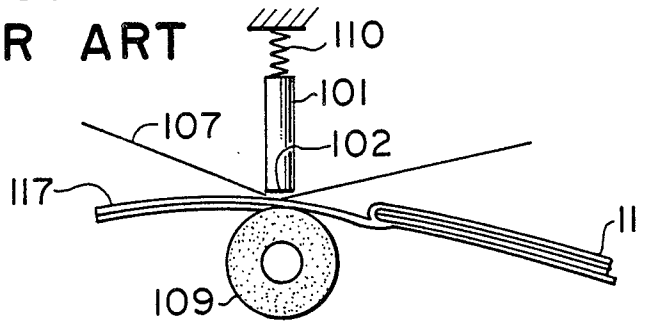
FIG. 5 PRIOR ART
