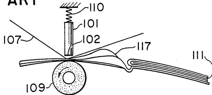
FIG. 5 PRIOR ART
