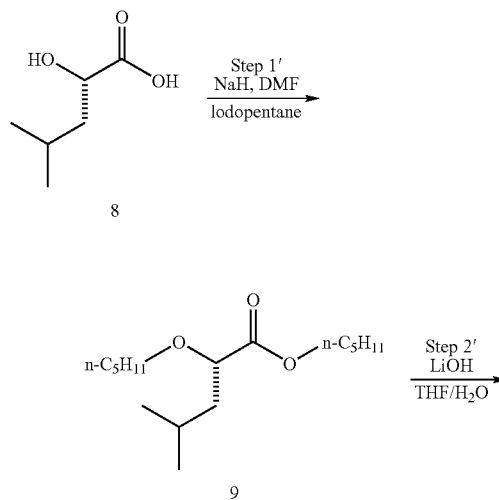
Scheme 8
