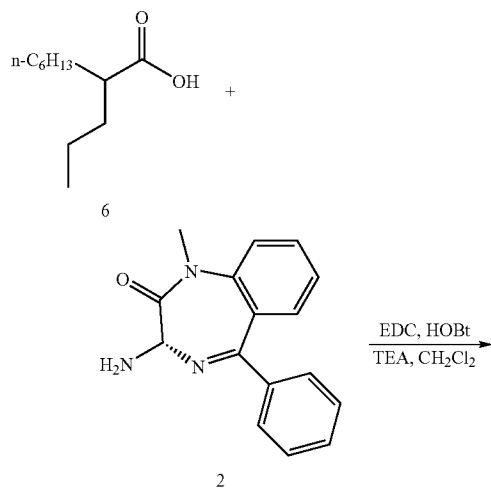
Scheme 7
