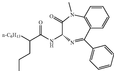
(3S)-3-[(1-oxo-2-propyloctyl)]amino-1-methyl-5-phenyl-2,3-dihydro-1H-1,4-benzodiazepin-2-one
