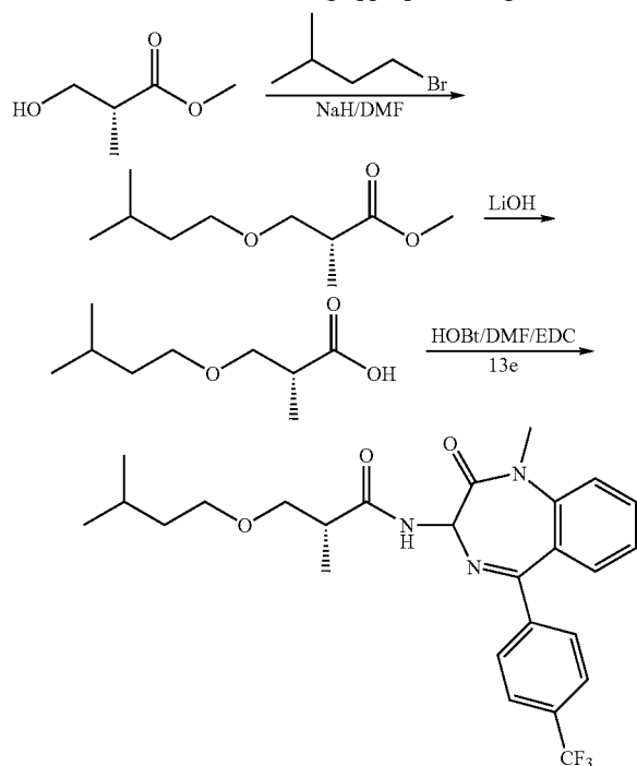
Example 15
