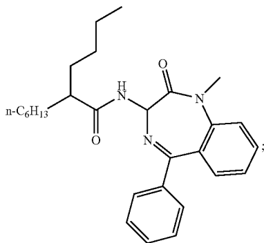
(3S)-3-[(1-oxo-2-butyloctyl)]amino-1-methyl-5-phenyl-2,3-dihydro-1H-1,4-benzodiazepin-2-one
