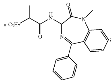
(3S)-3-[(1-oxo-2-methylpentyl)]amino-1-methyl-5-phenyl-2,3-dihydro-1H-1,4-benzodiazepin-2-one
