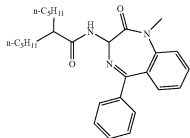
(3S)-3-[(1-oxo-2-propylpentyl)]amino-1-methyl-5-phenyl-2,3-dihydro-1H-1,4-benzodiazepin-2-one
