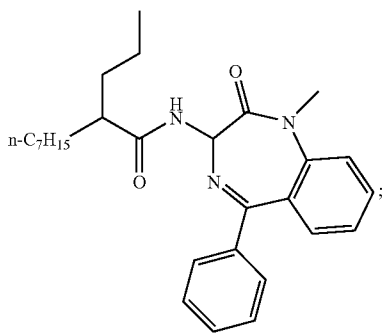
(3S)-3-[(1-oxo-2-butyloctyl)]amino-1-methyl-5-phenyl-2,3-dihydro-1H-1,4-benzodiazepin-2-one
