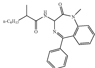
(3S)-3-[(1-oxo-2-pentylheptanyl)]amino-1-methyl-5-phenyl-2,3-dihydro-1H-1,4-benzodiazepin-2-one
