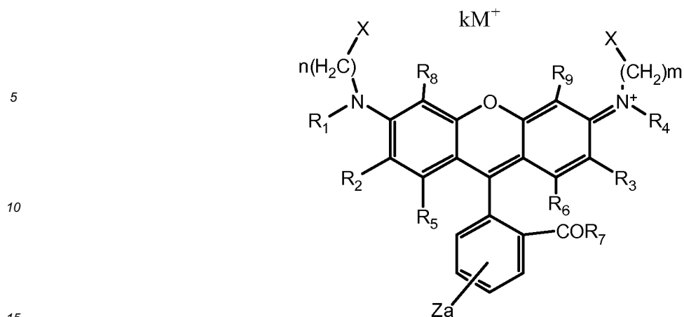
Formula (I)
