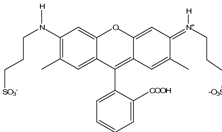
Dye 1
