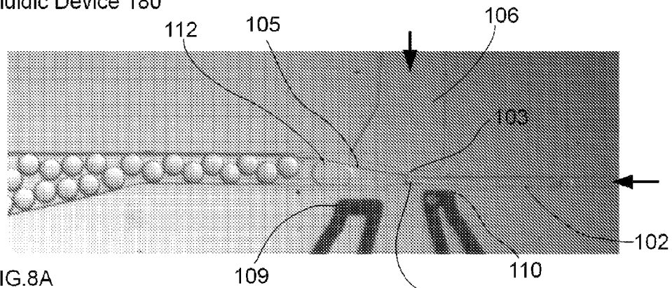
Microfluidic Device 180
