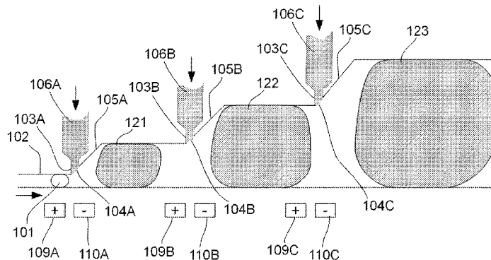
Microfluidic Device 120
