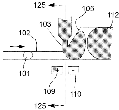
Microfluidic Device 240, SECTION 125A
