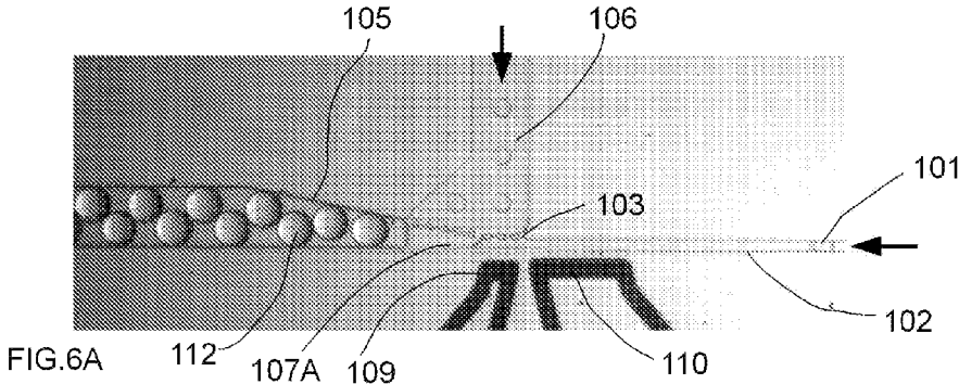
Microfluidic Device 140
