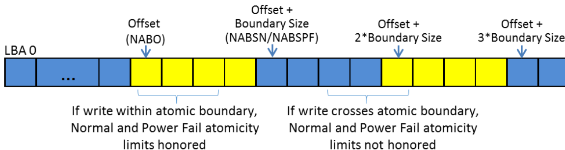
Figure 195: Atomic Boundaries Example
