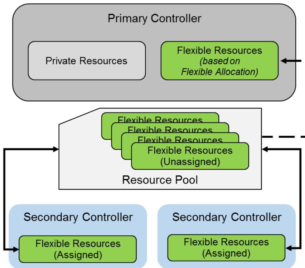
Figure 265: Controller Resource Allocation
