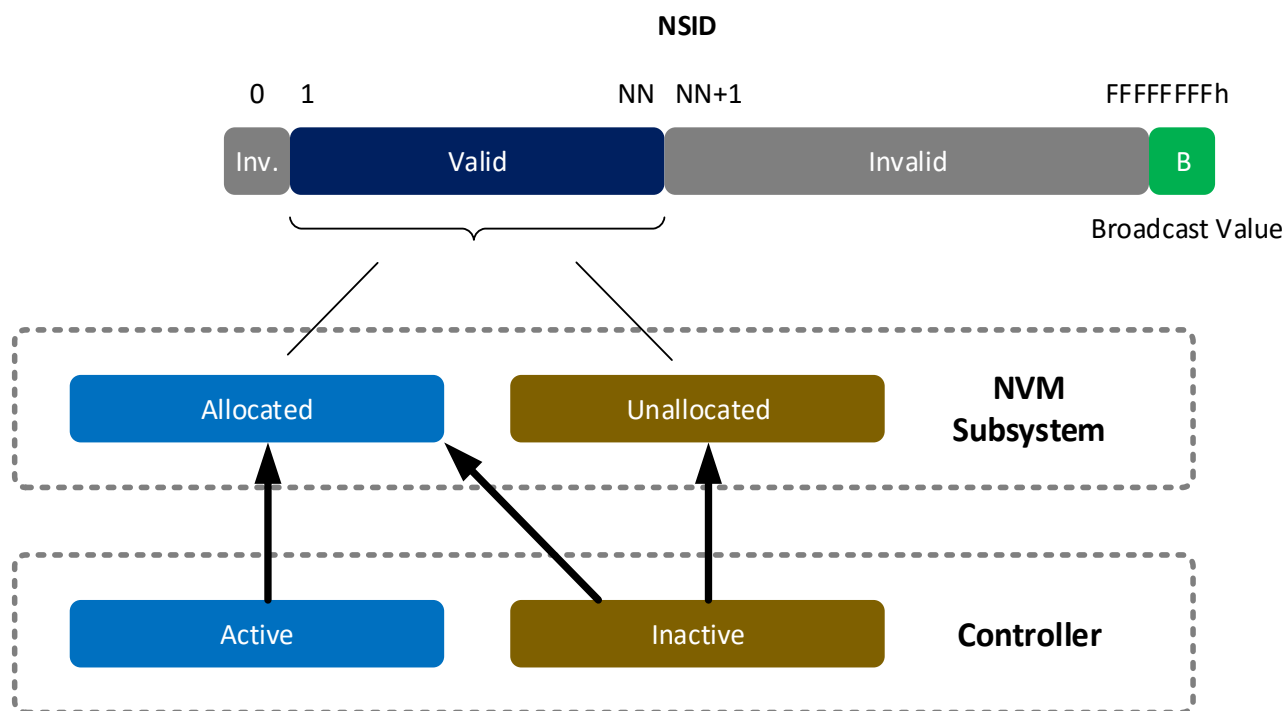
Figure 189: NSID Types
