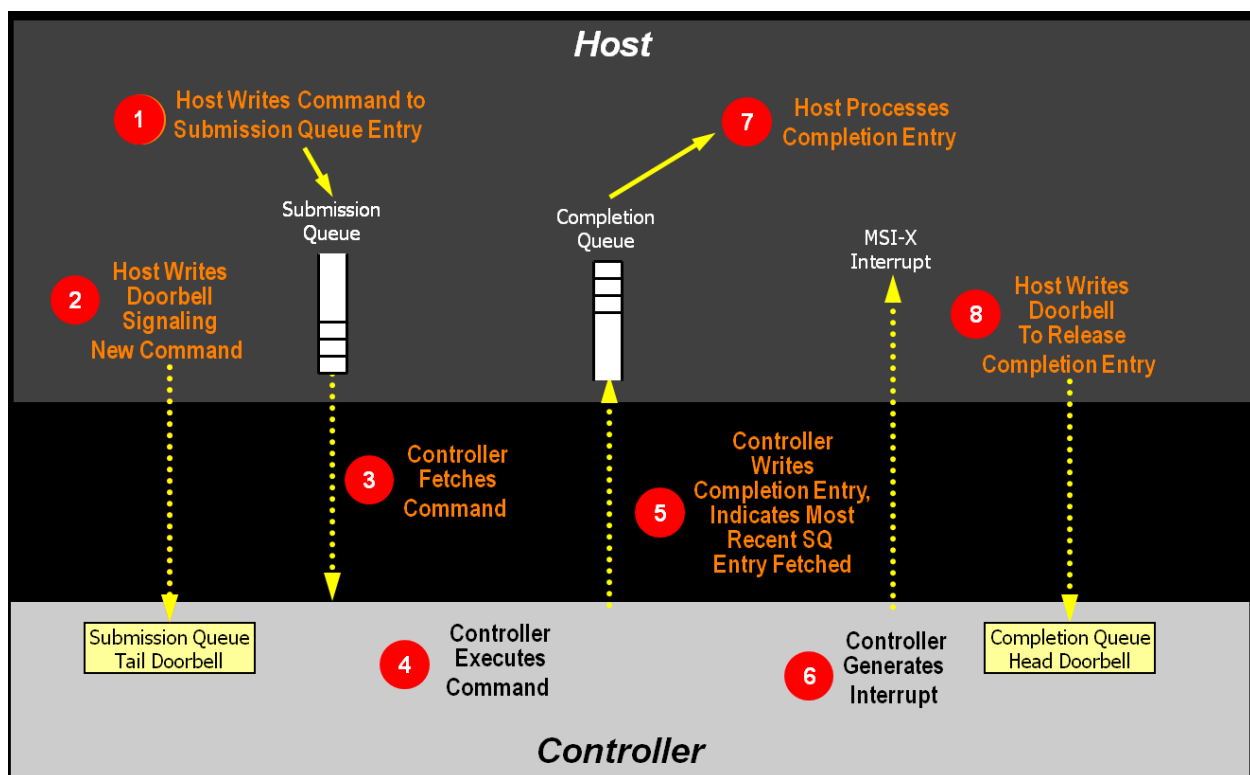
Figure 251: Command Processing
