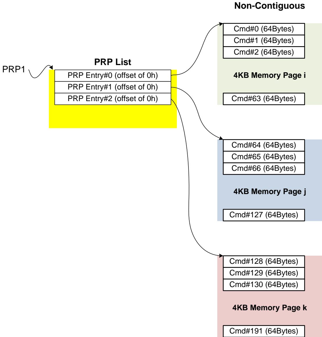
Figure 252: PRP List Describing I/O Submission Queue
