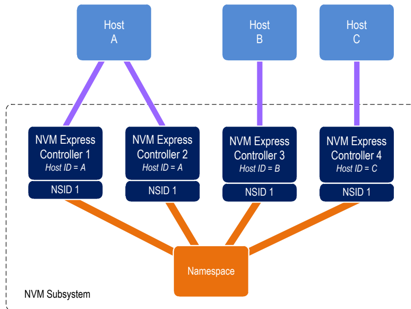
Figure 266: Example Multi-Host System
