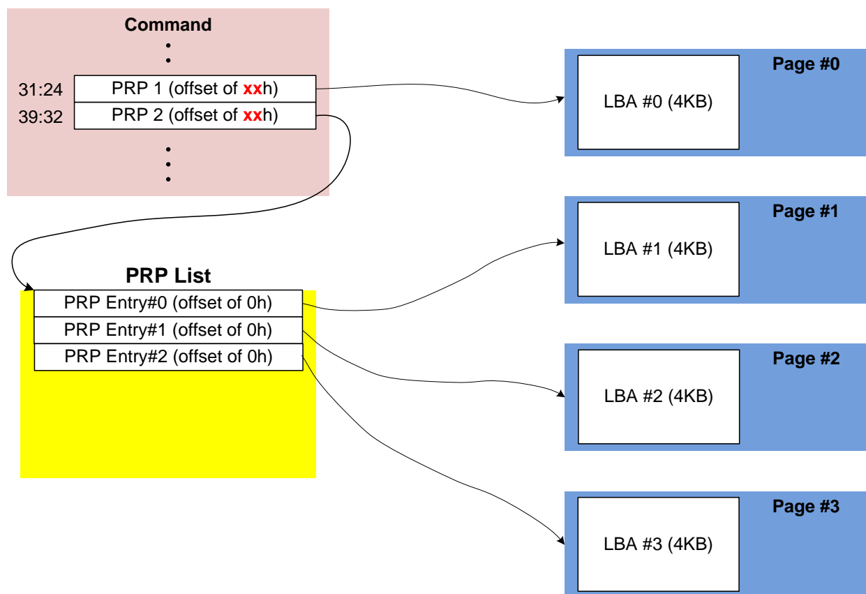
Figure 253: PRP List Describing Data to Compare
