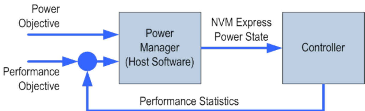
Figure 261: Dynamic Power Management
