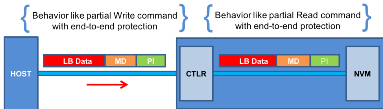
Figure 260: Protection Information Processing for Compare
