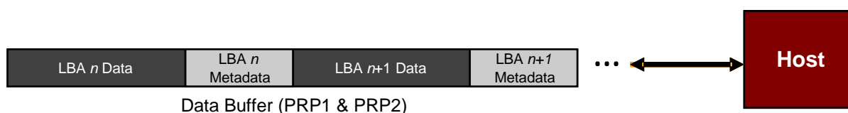
Figure 255: Metadata – Contiguous with LBA Data, Forming Extended LBA
