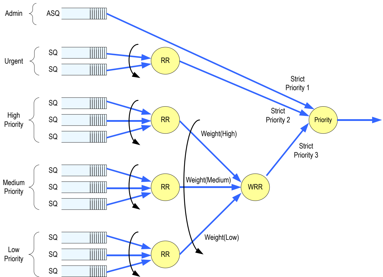
Figure 40: Weighted Round Robin with Urgent Priority Class Arbitration
