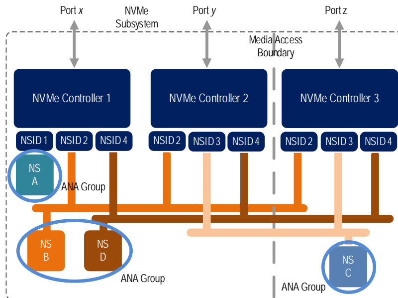
Figure 493: Multiple Namespace groups
