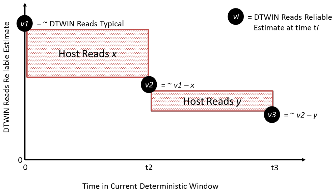
Figure 487: Typical and Reliable Estimate Example
