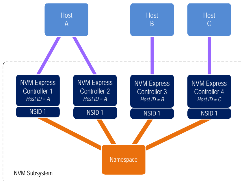
Figure 460: Example Multi-Host System
