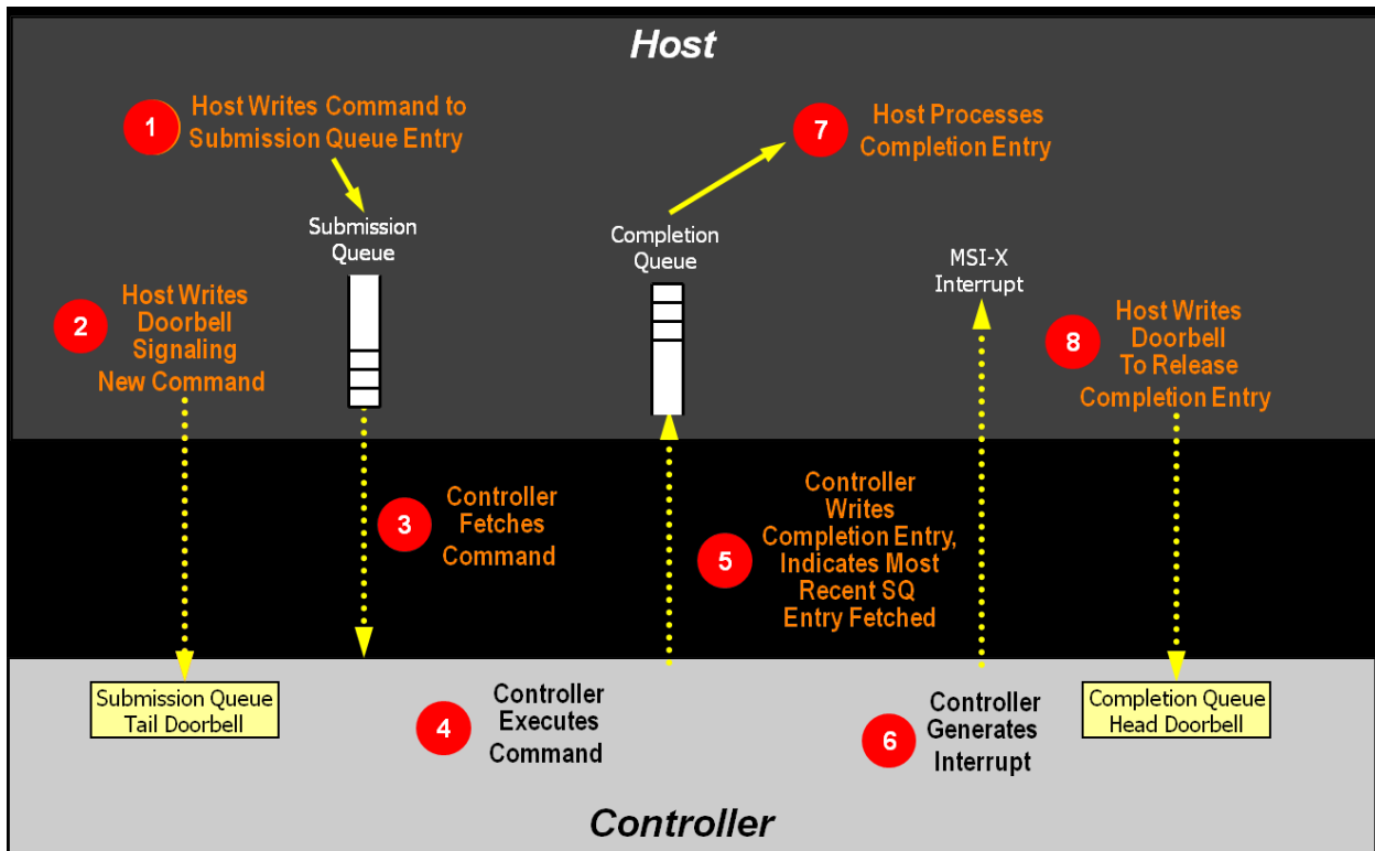
Figure 432: Command Processing
