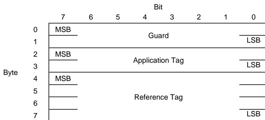
Figure 451: Protection Information Format
