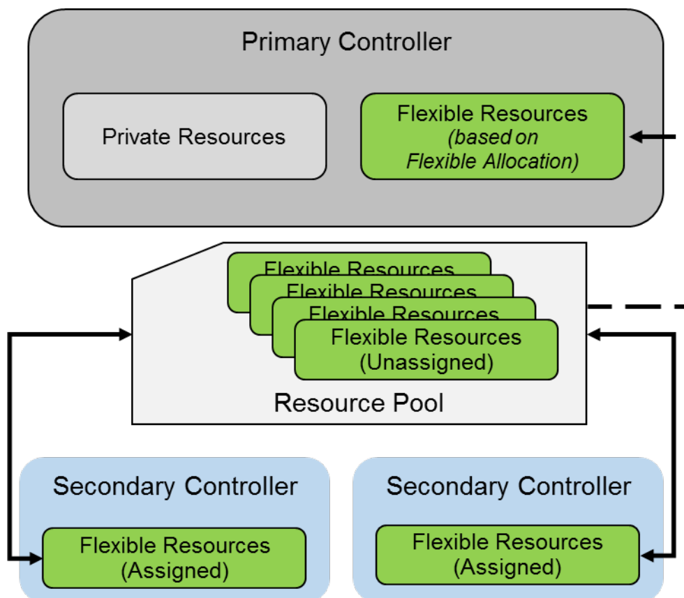
Figure 459: Controller Resource Allocation
