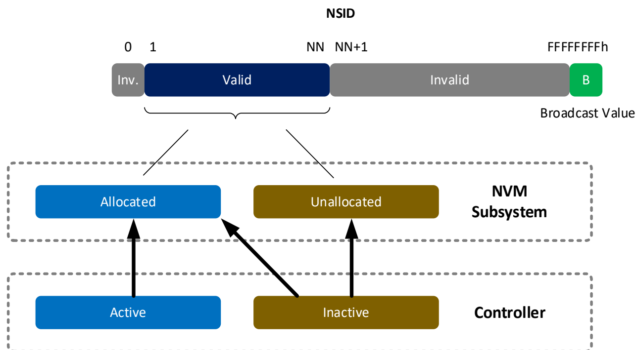
Figure 348: NSID Types
