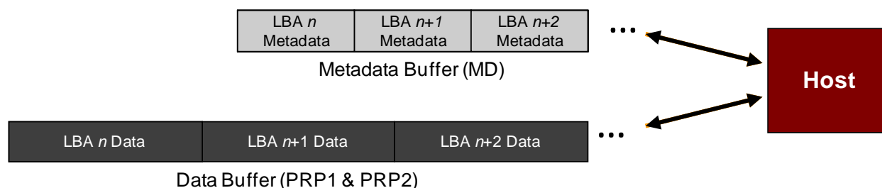
Figure 450: Metadata – Transferred as Separate Buffer
