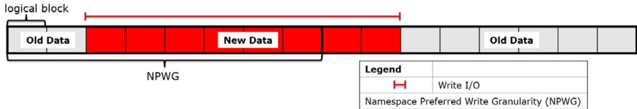
Figure 504: Host write I/O command following NPWG but not NPWA attributes
