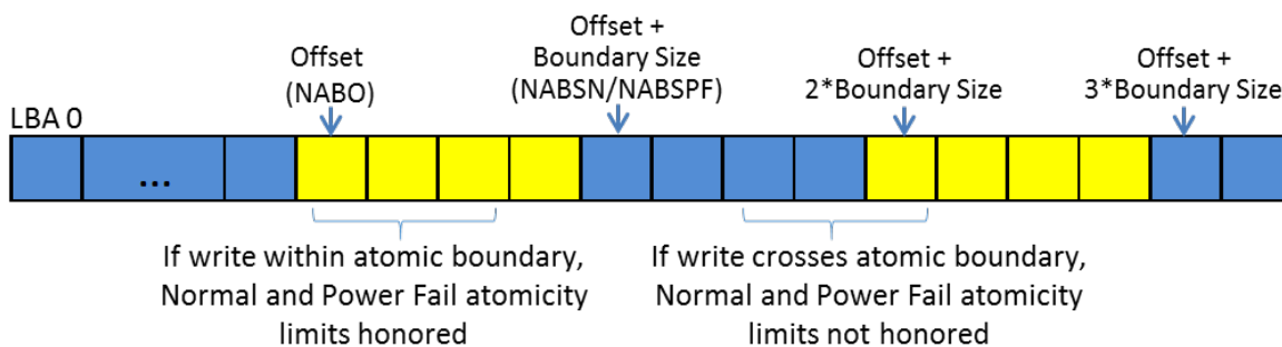
Figure 354: Atomic Boundaries Example
