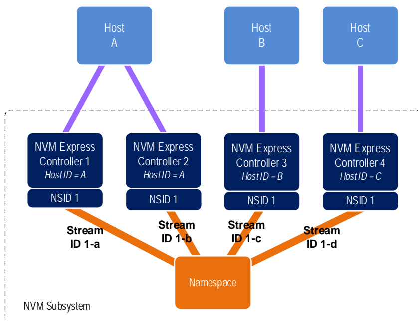
Figure 513: Example Multi-Stream and NSSC
