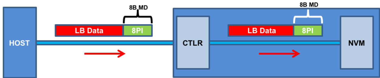
Figure 452: Write Command Protection Information Processing
