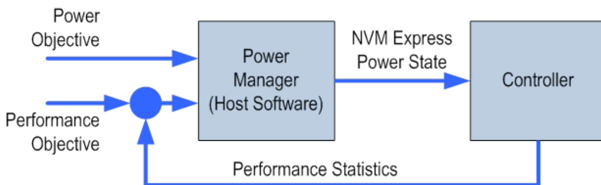
Figure 455: Dynamic Power Management
