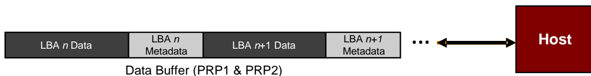
Figure 449: Metadata – Contiguous with LBA Data, Forming Extended LBA
