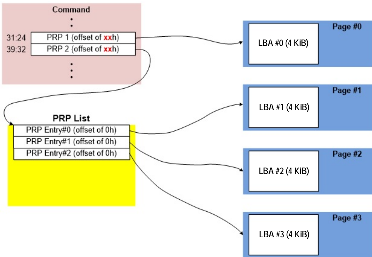
Figure 434: PRP List Describing Data to Compare
