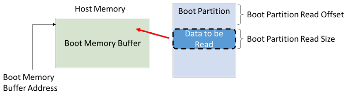
Figure 476: Boot Partition Overview
