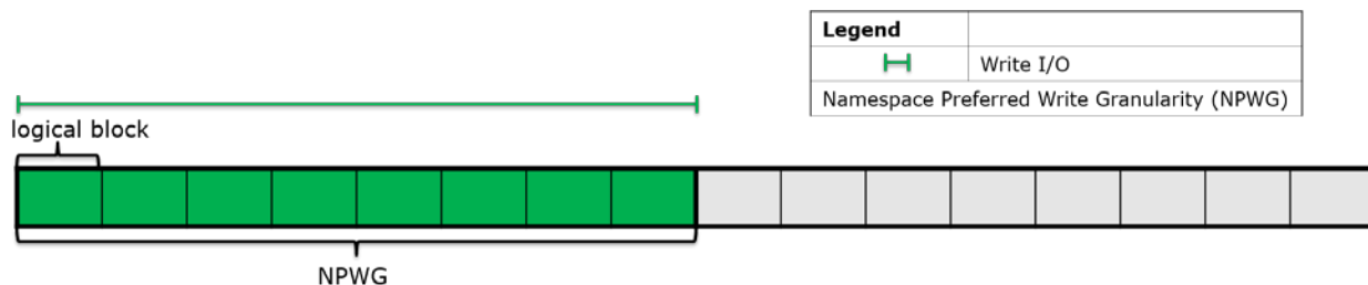
Figure 503: Host write I/O command following NPWA and NPWG
