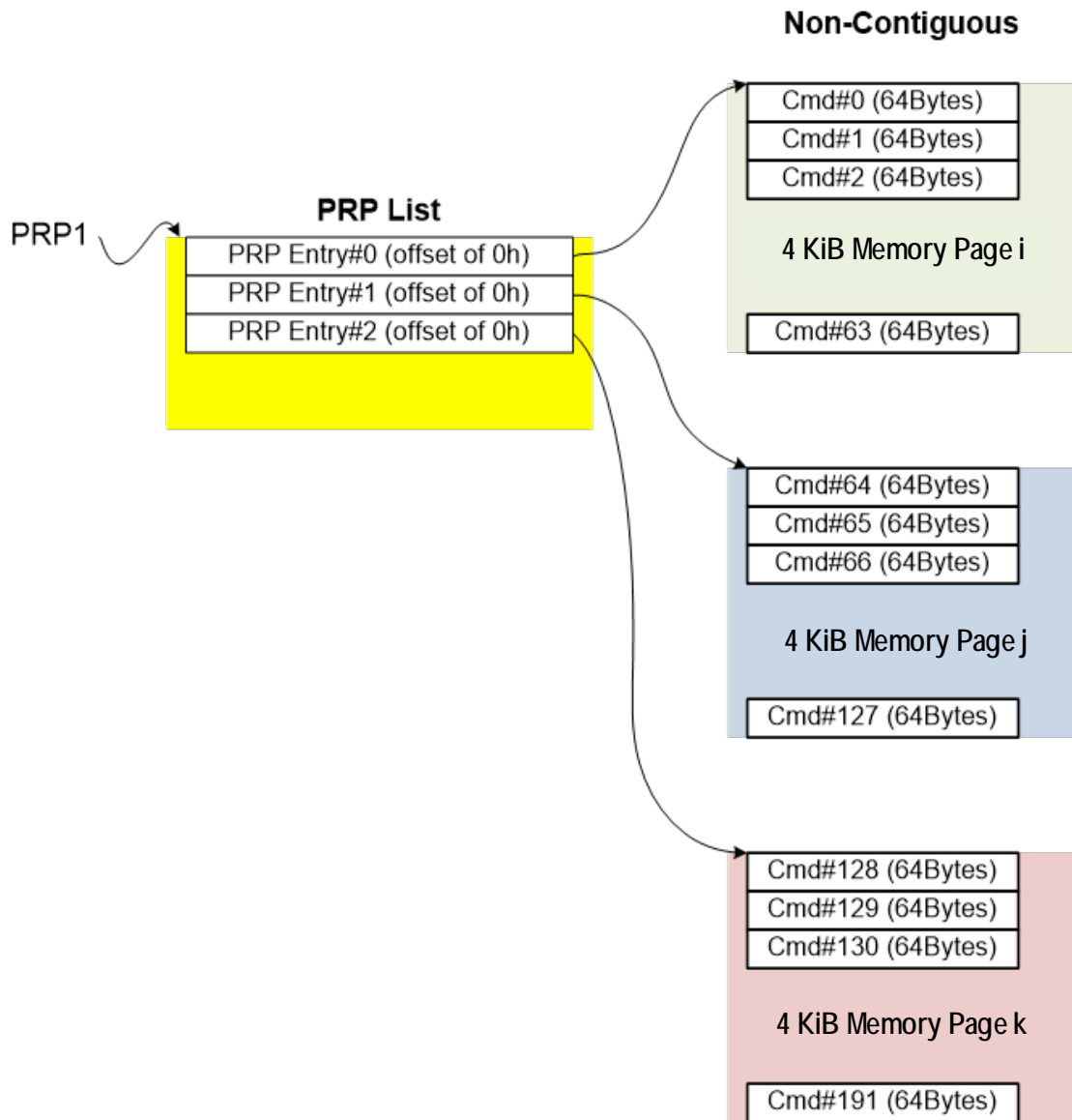
Figure 433: PRP List Describing I/O Submission Queue
