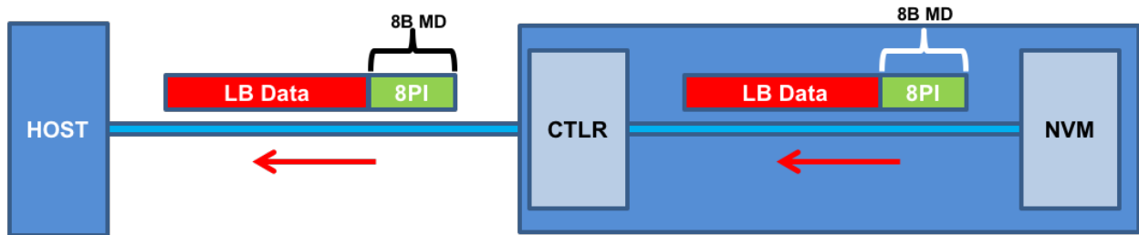
Figure 453: Read Command Protection Information Processing
