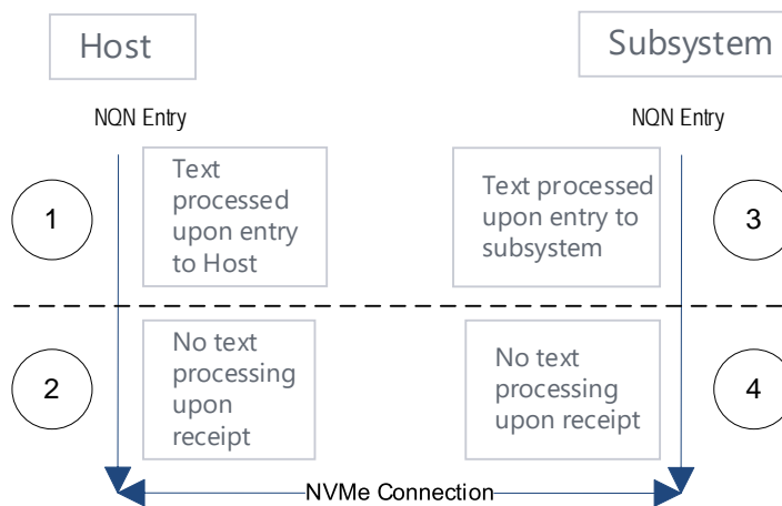
Figure 436: NQN Processing
