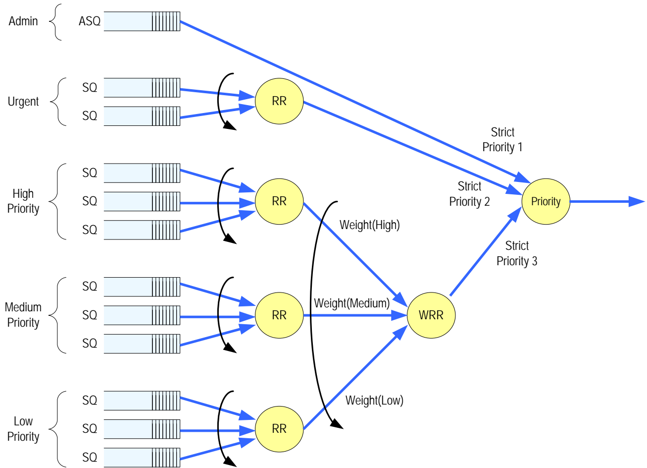
Figure 138: Weighted Round Robin with Urgent Priority Class Arbitration
