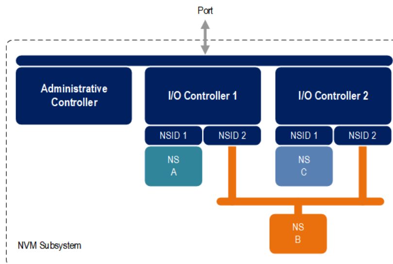
Figure 424: NVM Subsystem with One Administrative and Two I/O Controllers
