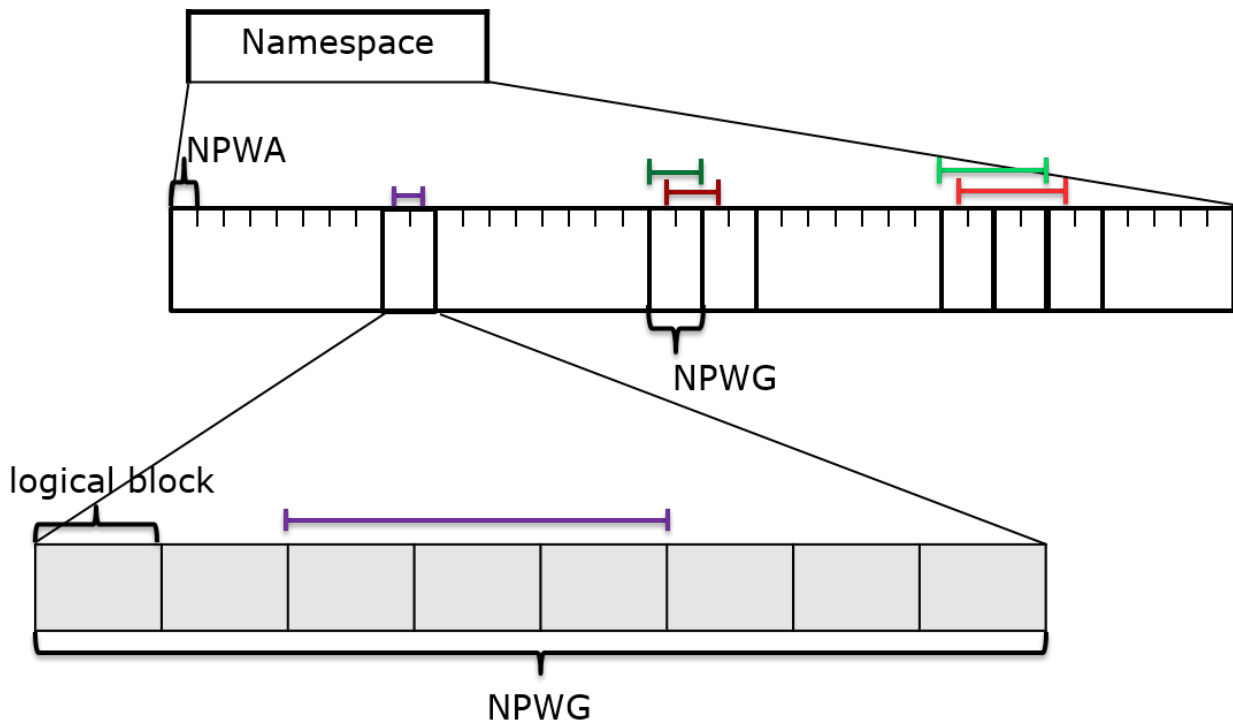
Figure 501: Example namespace broken down to illustrate potential NPWA and NPWG settings
