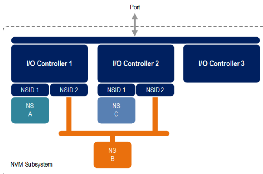
Figure 416: NVM Subsystem with Three I/O Controllers
