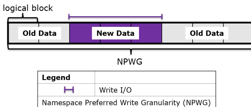
Figure 502: Non-conformant Write Impact
