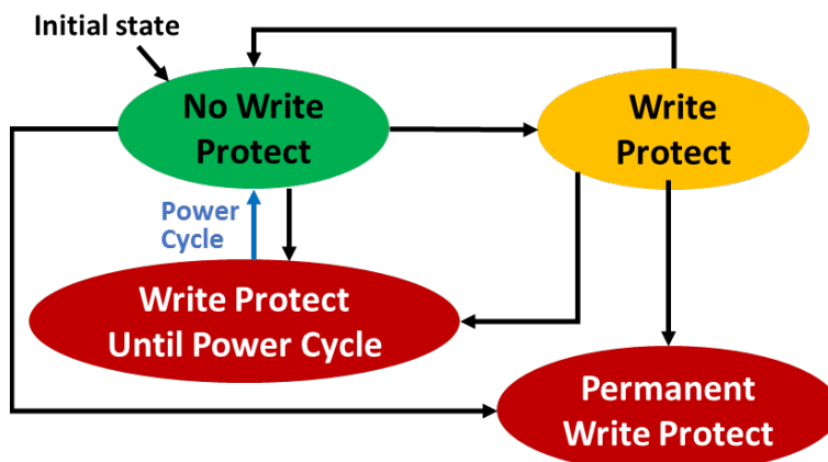
Figure 489: Namespace Write Protection State Machine Model
