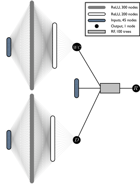
Fig. 4. The proposed detection scheme is a combination of two NNs regression models and one random forest with 100 trees. The two NNs are trained independently to evaluate the water content and the depth of the rebar based on the compressed signal. Subsequently, the estimated water content and depth are combined with the compressed A-scan and used as inputs for RF. The output of the random forest is the estimated radius of the rebar.
