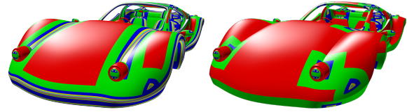
Figure 3: Car model consisting of 1519 patches with 314 semi-smooth crease tags (sharpness of 6) rendered with feature adaptive subdivision (left) and our method (right). Subdivision levels are indicated by different colors.
