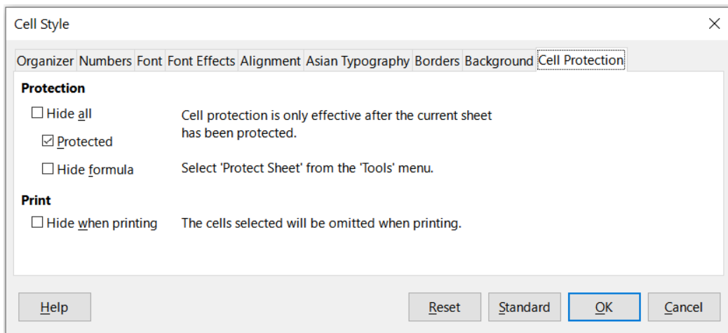
Figure 201: Cell Style dialog – Cell Protection tab
