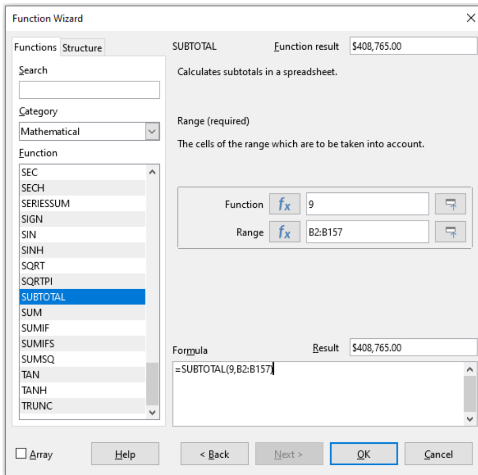
Figure 350: Function Wizard dialog
