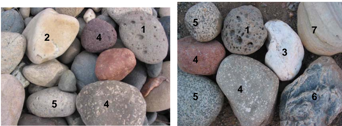
Figure 11. Different types of pebbles in gravel. 1, volcanic lava with gas bubbles. 2, quartzite. 3, quartz. 4, volcanic lava. 5, granitic rock. 6, chert. 7, mudstone.
